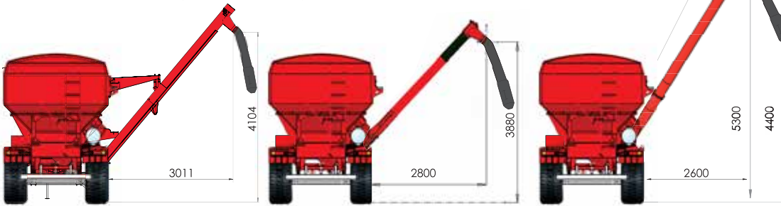
LOADING AND INOCULATING AUGER
