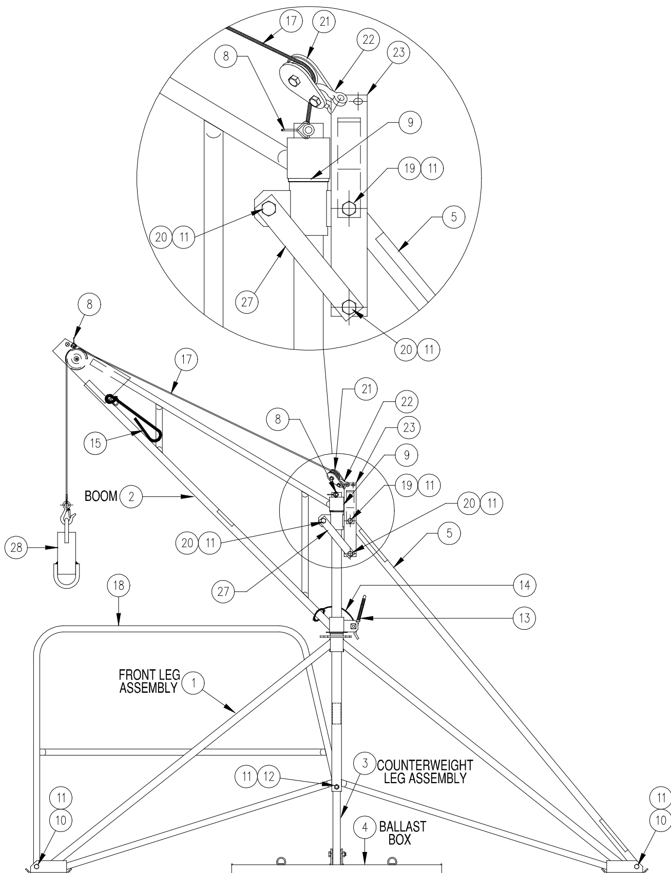
Figure 8-3 SH300 w/ Handwinch Assembly—Front View
