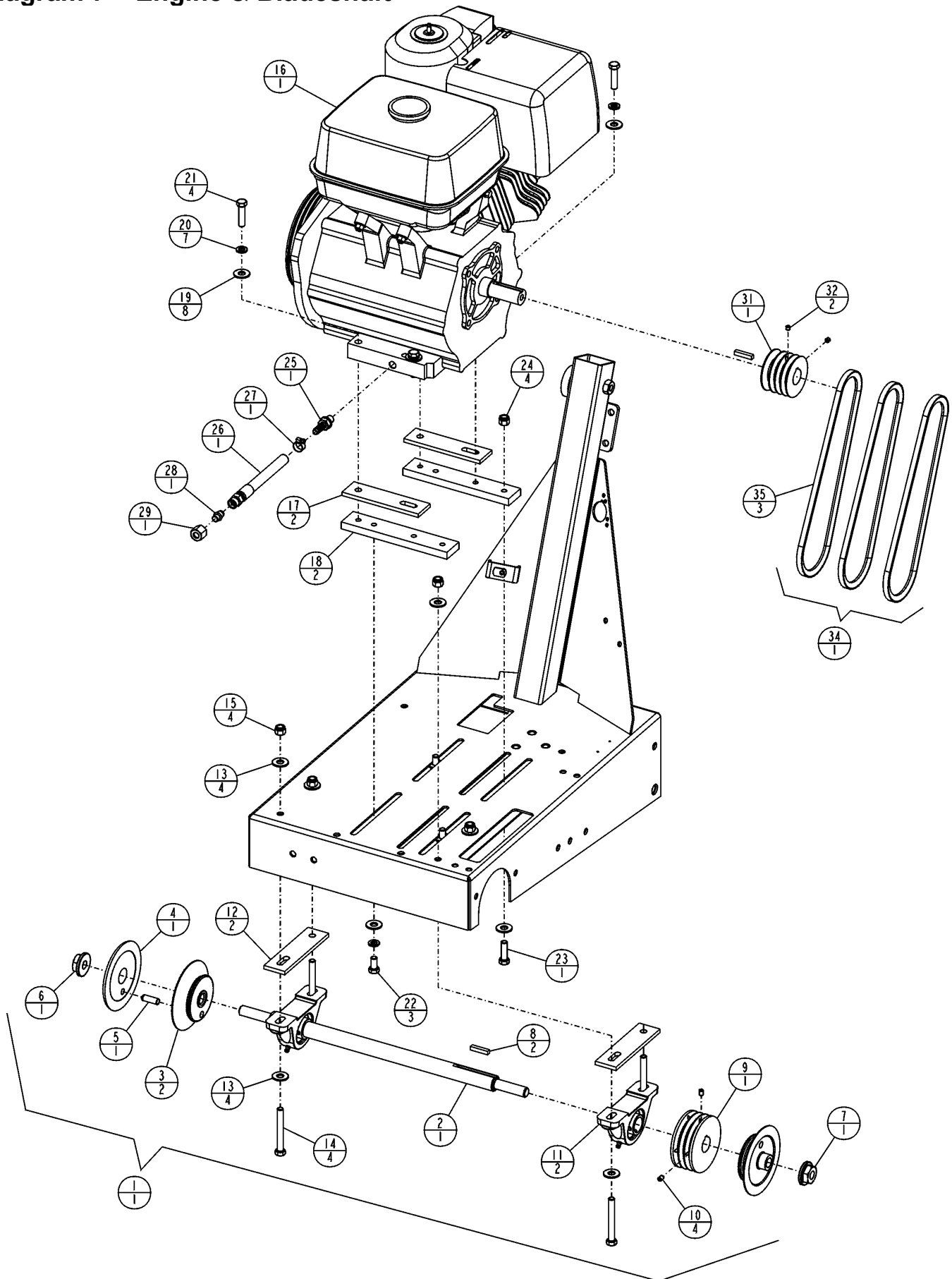
Diagram 7 – Engine & Bladeshaft
