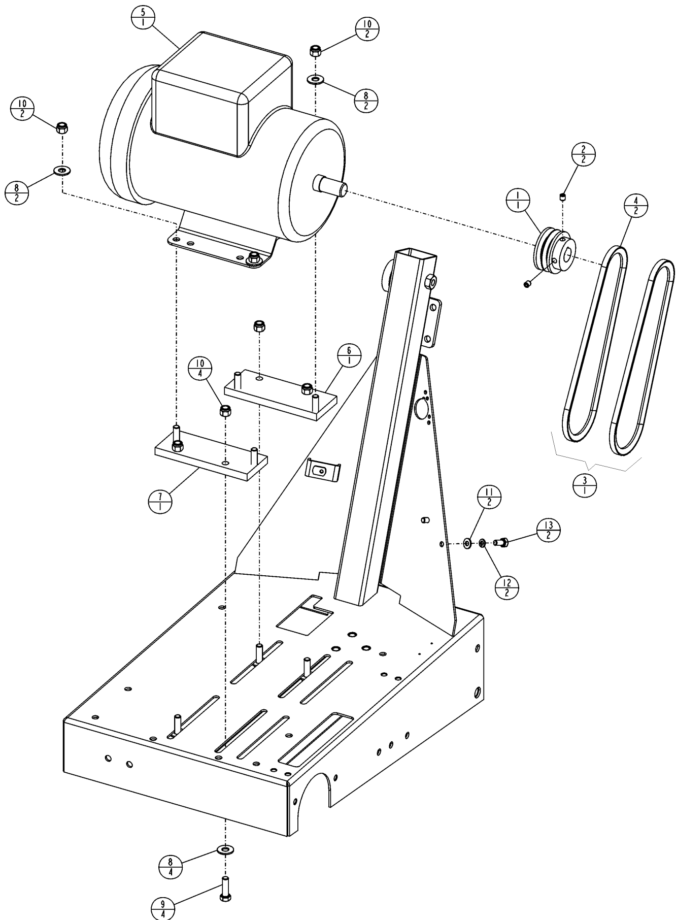
Diagram 8 – Electric Motor
