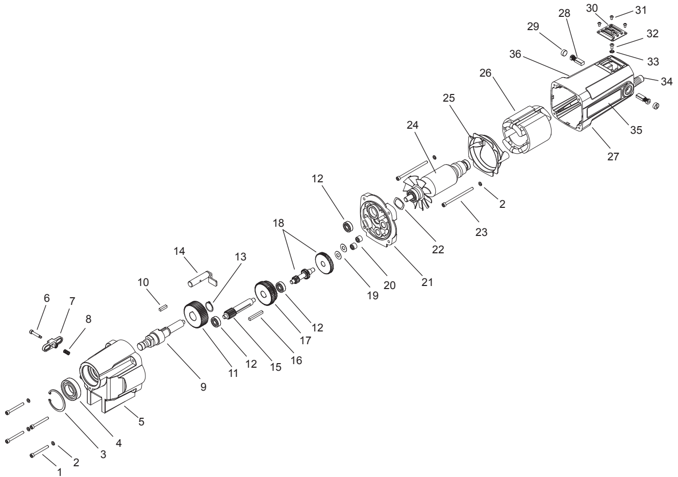
08141 Motor Assembly
