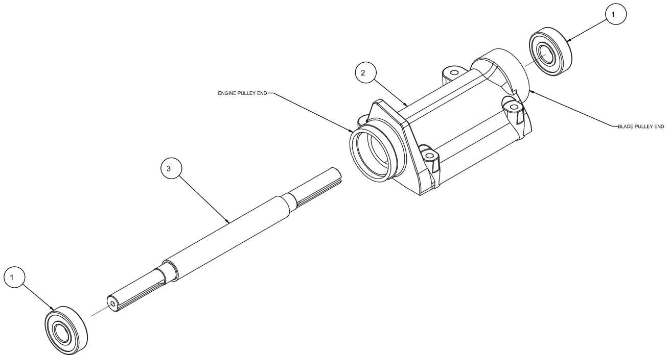
FIGURE 20 - MK-5000 ASSY, JACK SHAFT P/N 166045
