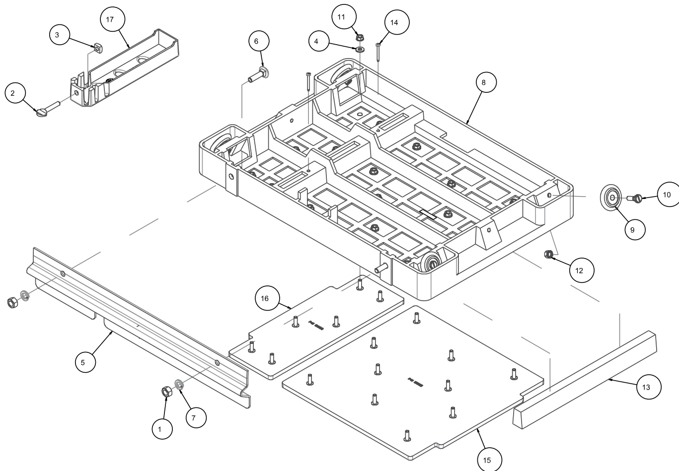
FIGURE 19 - MK-5000 ASSY, TABLE P/N 152124
