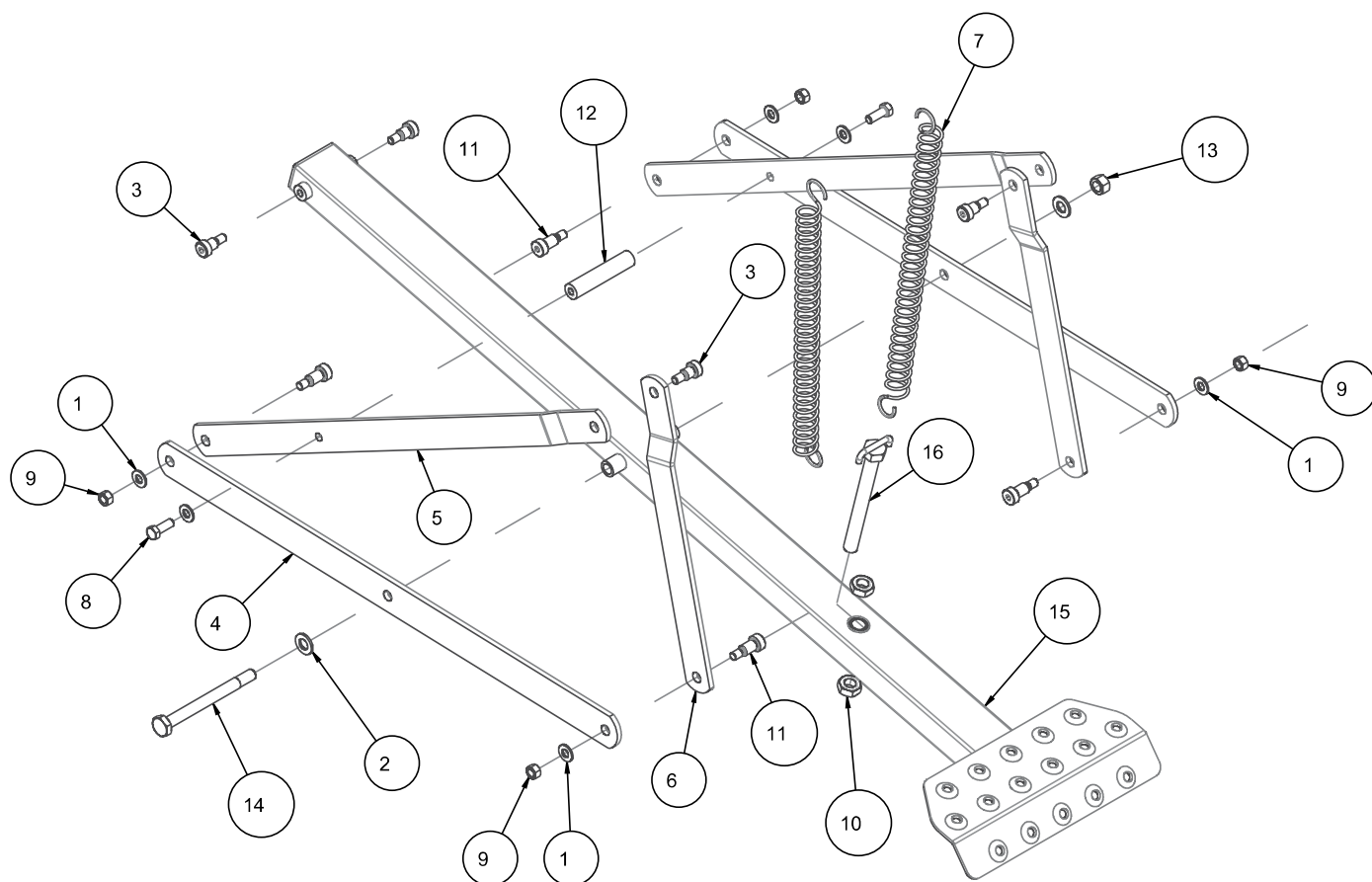
FIGURE 9 - MK-5000 ASSY, BLOCK SAW FOOTPEDAL P/N 154629
