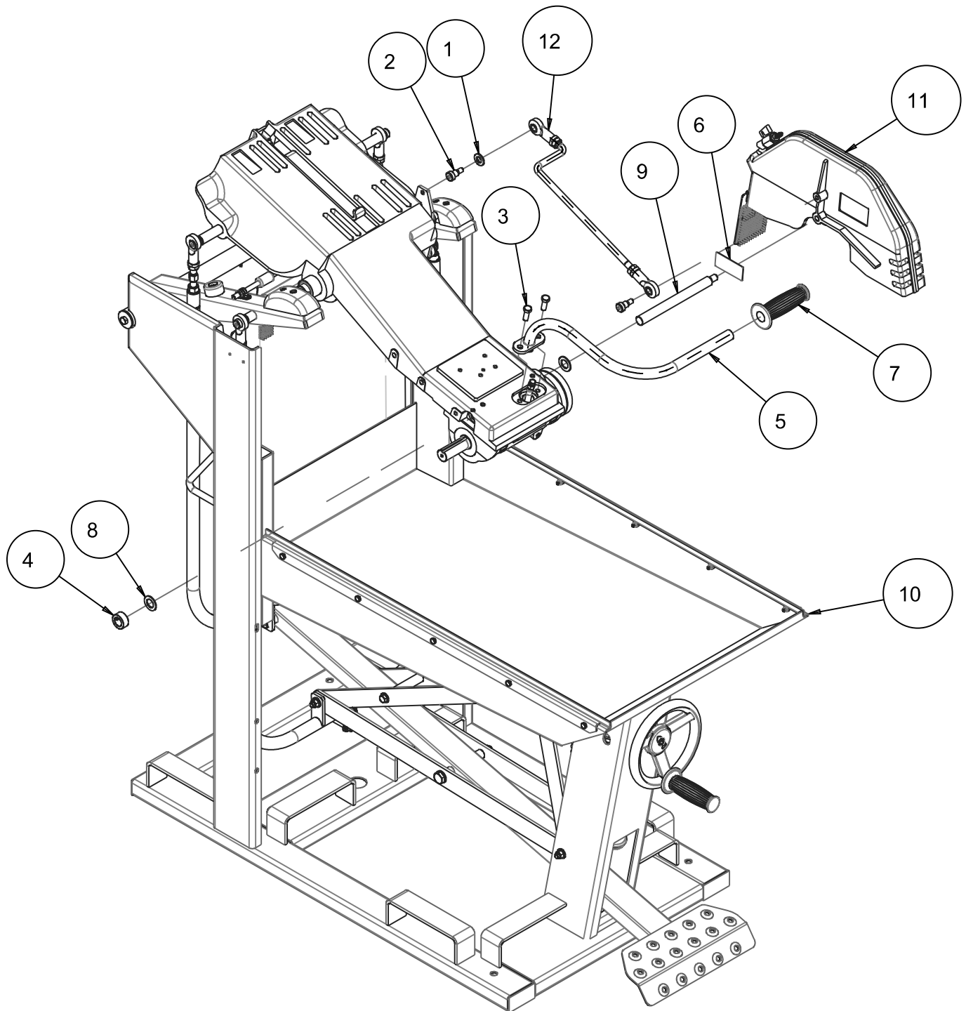
FIGURE 4 - MK-5000 BLOCK SAW 14IN BLADE GUARD P/N 172446-14
