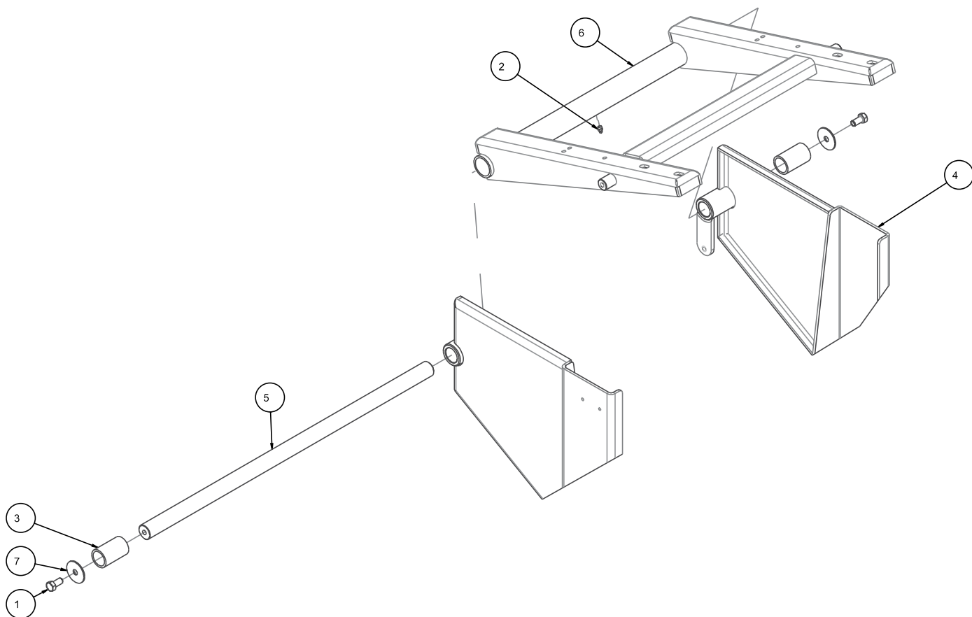
FIGURE 7 - MK-5000 ASSY, BLOCK SAW ELEVATOR ARM P/N 154629
