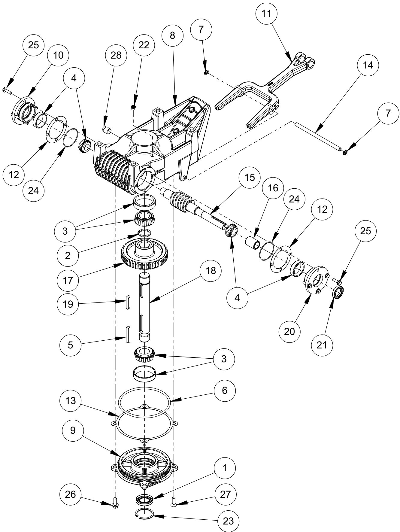
Gearbox Assembly
