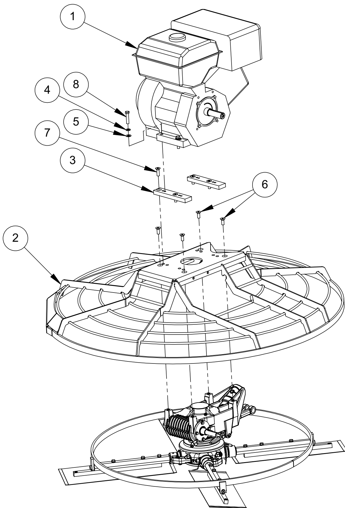
Guard Assembly
