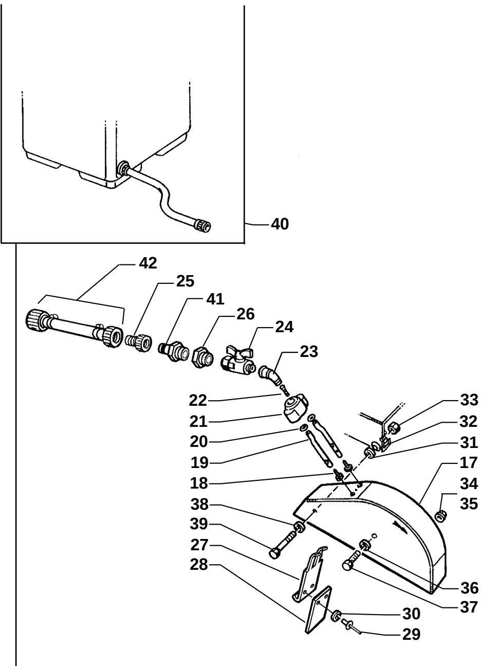
FIGURE 3 - Blade Shaft & Blade Guard Group
