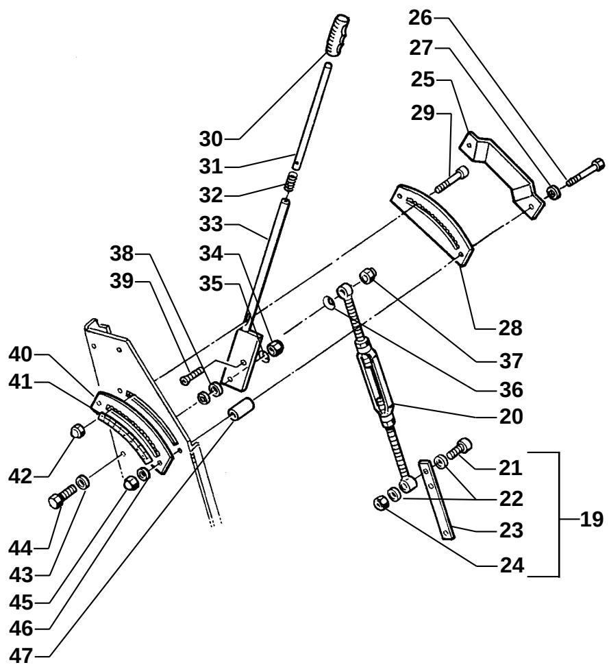
FIGURE 2 - Pointer, Depth Control Group
