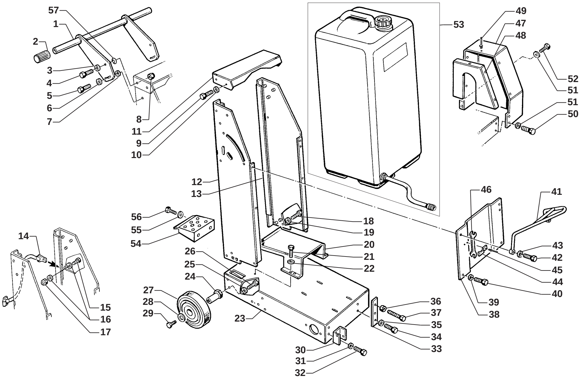
FIGURE 1 - Frame Group
