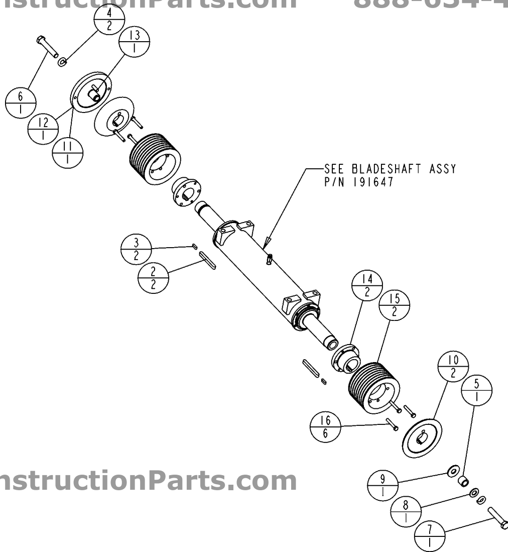
Diagram 31 - Bladeshaft Group, 36" Drive, 198091
