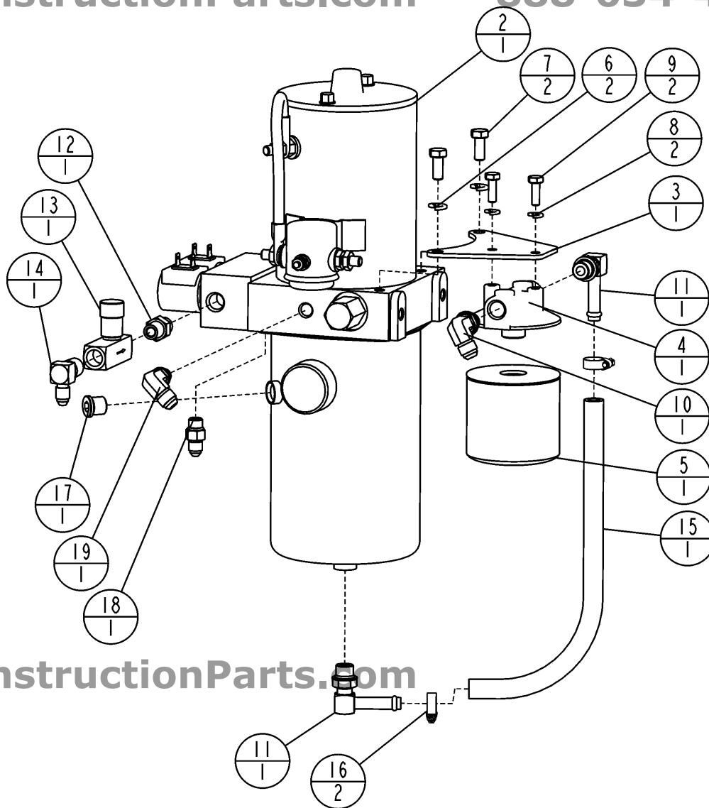
Diagram 16 - Lift Pump Assembly, 191969
