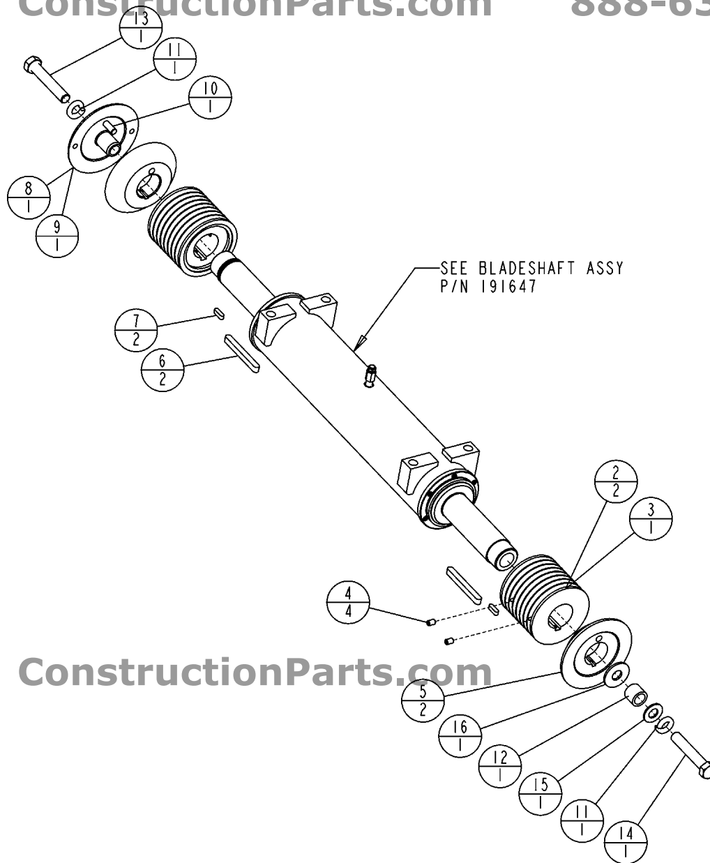
Diagram 29 - Bladeshaft Group, 18" Drive, 198089
