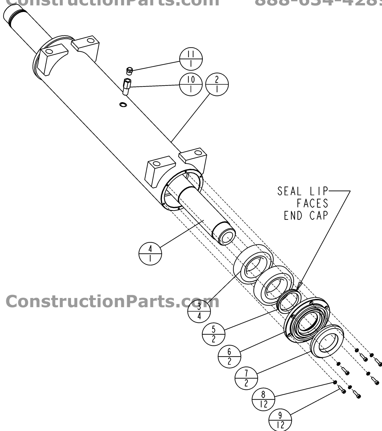
Diagram 28 - Bladeshaft Assembly, 191647
