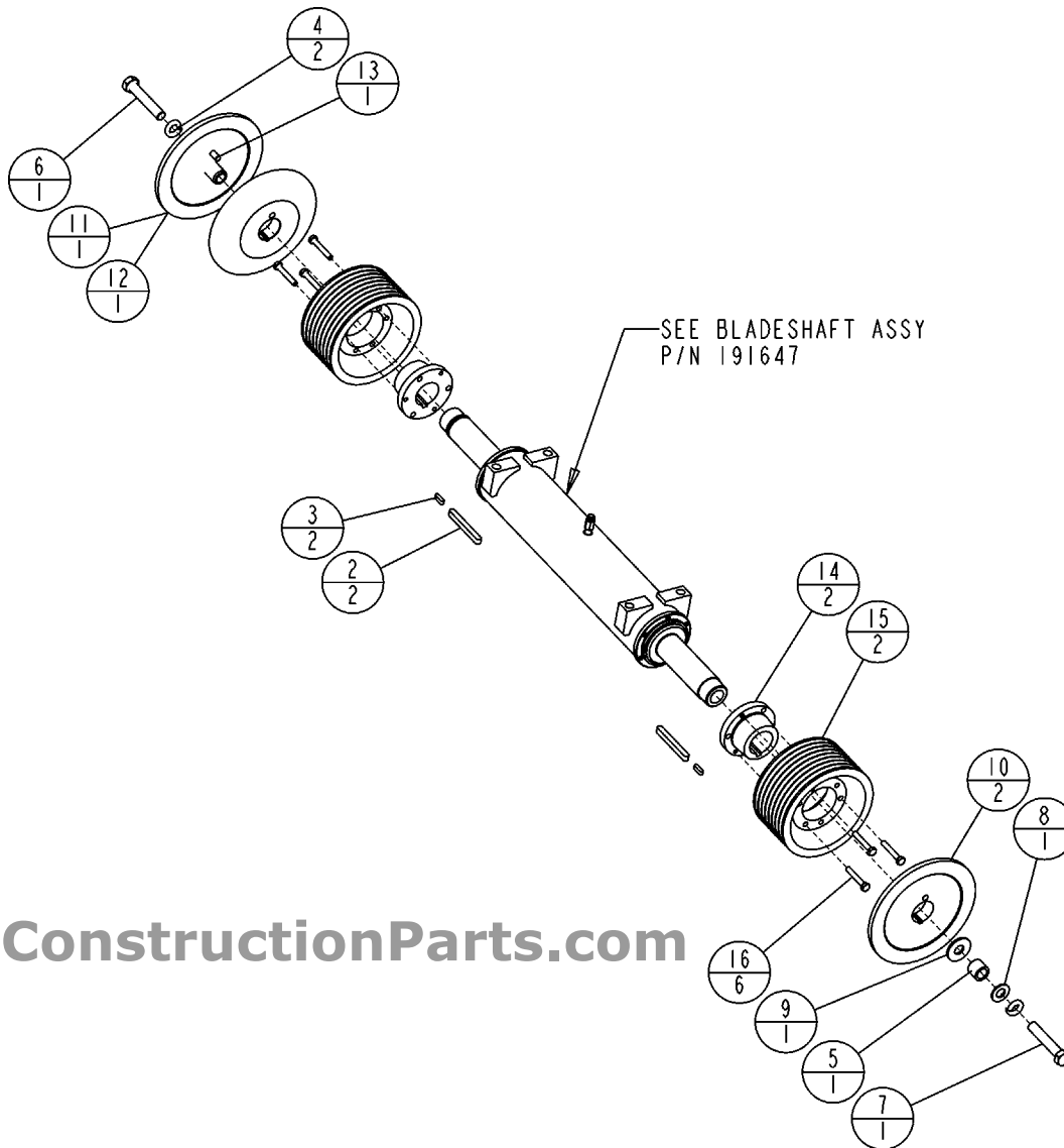
Diagram 32 - Bladeshaft Group, 48" Drive, 198092
