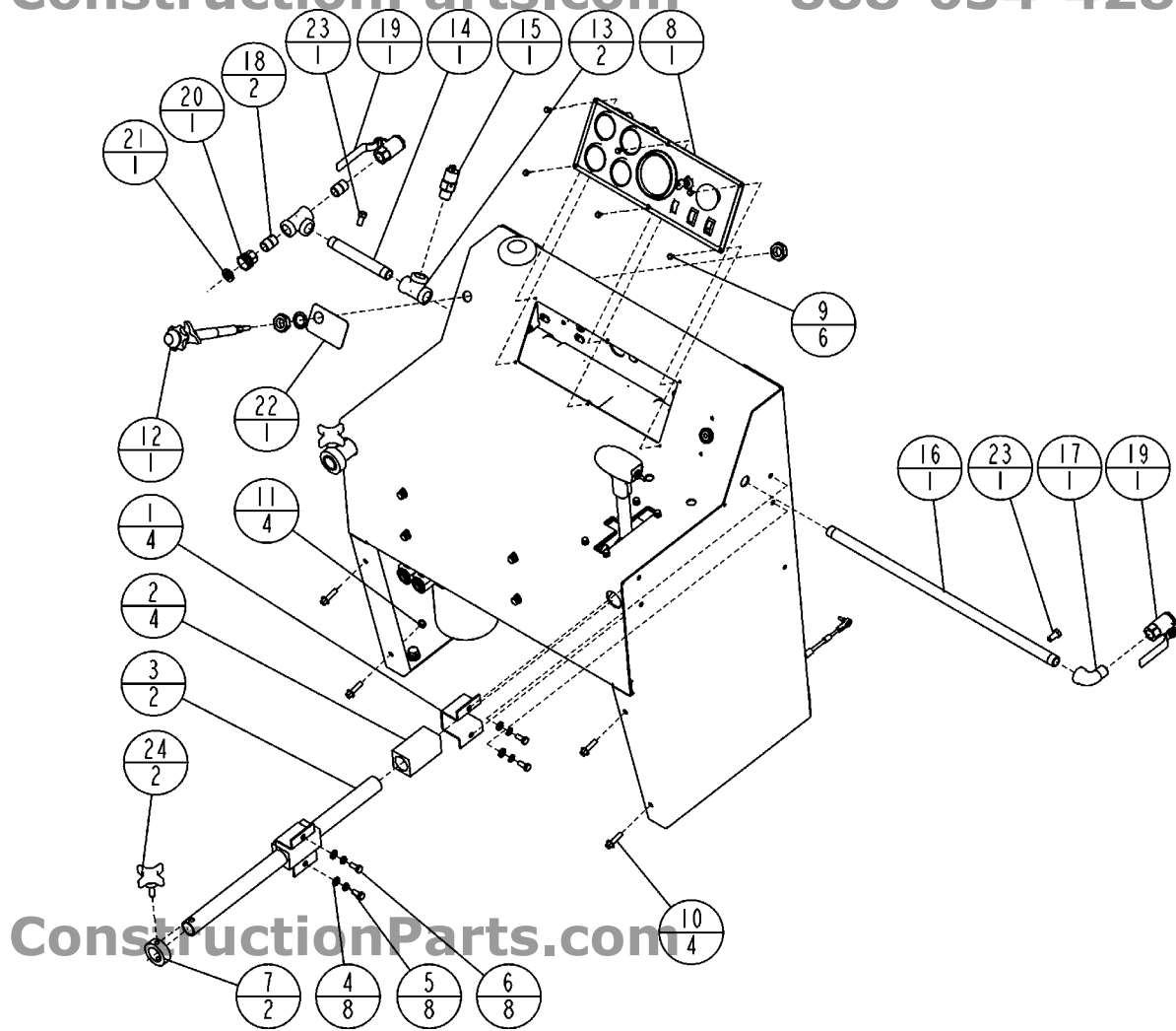
Diagram 8 - Cowl Assembly Group
