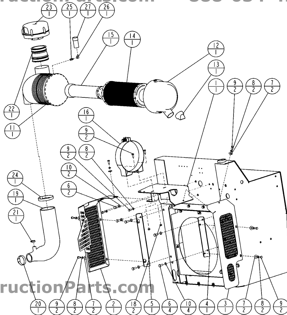
Diagram 27 - Air Cleaner Group, 198123
