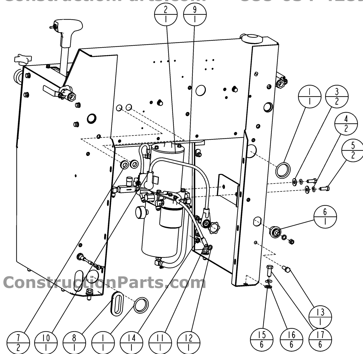
Diagram 15 - Lift Pump Group
