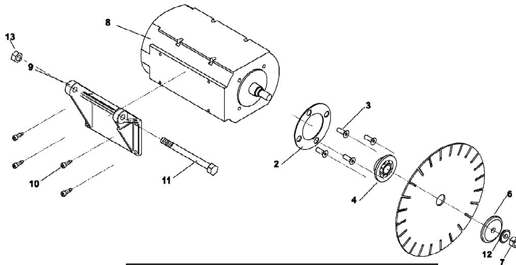
TAV. 2 ASSEMBLY OF MOTOR -
