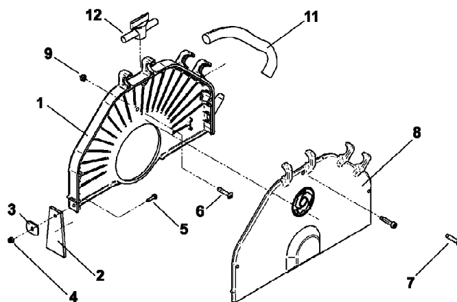
TAV. 3 - BLADE GUARD
