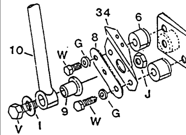
Engine Recoil Side Handle Assembly
