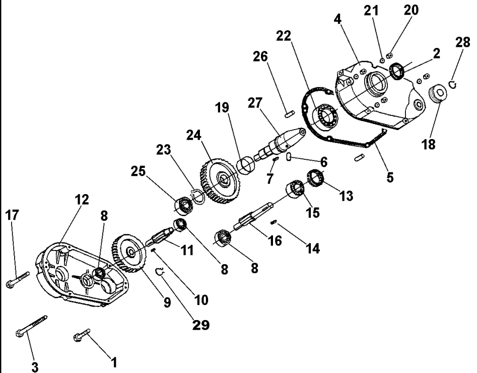
TAV. 8 - DRUM REDUCTION UNIT - WORKMAN II 350 (COD. 3209786)
