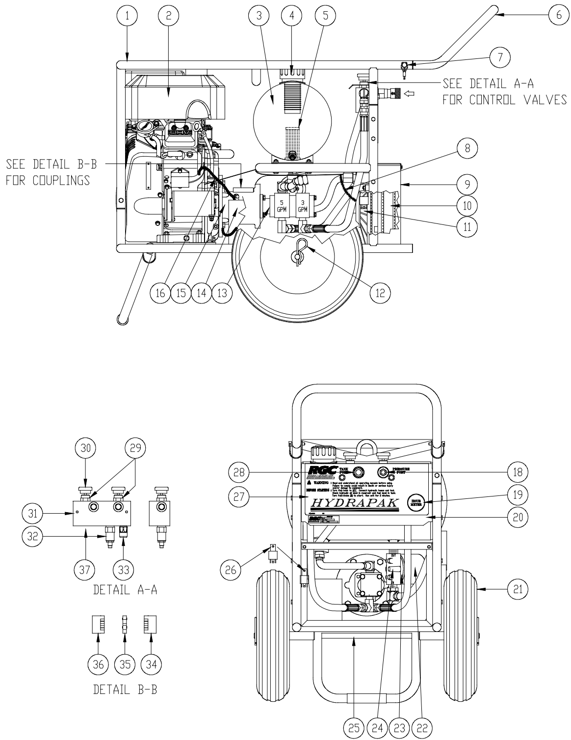
Figure 6-1. HH1358C, HV1658C, and HV1858C Assembly Drawing
