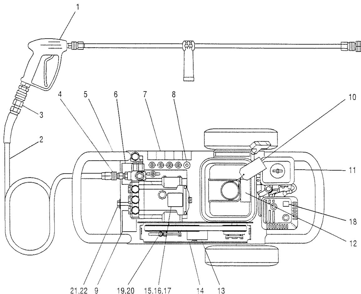
Figure 6 - Machine Assembly, Top View
