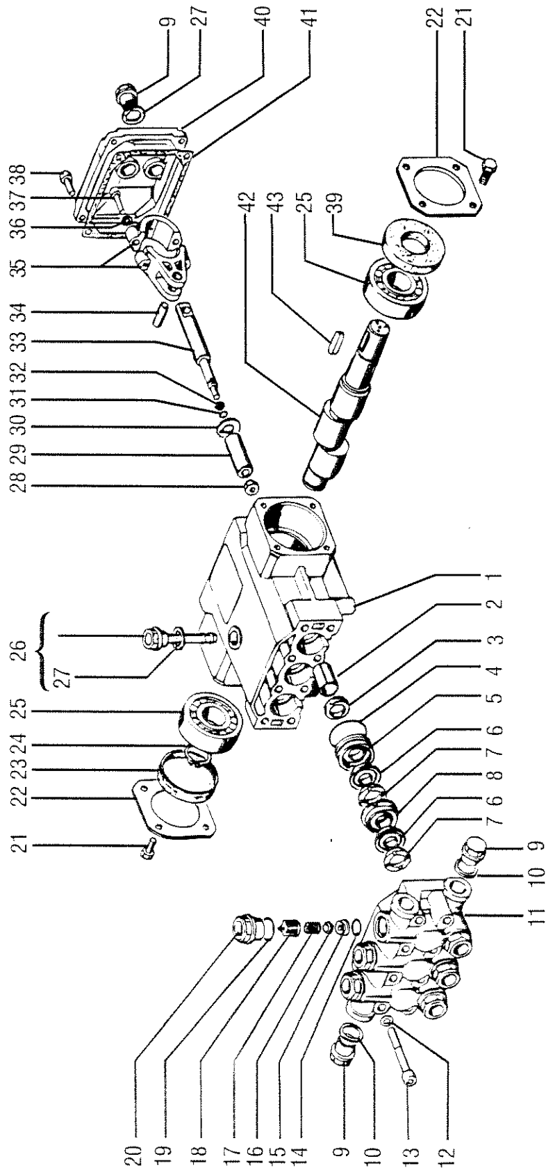
Figure 9 - Pump, Exploded View
