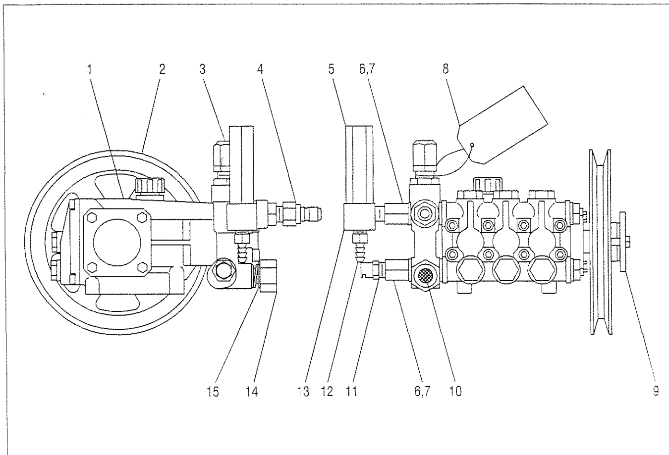
Figure 8 - Pump Assembly
