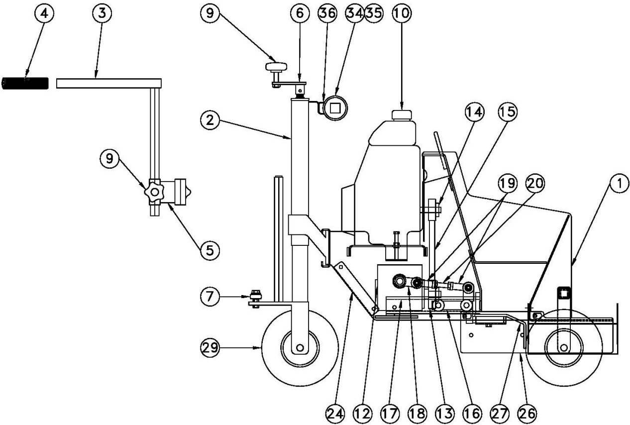
Side View
