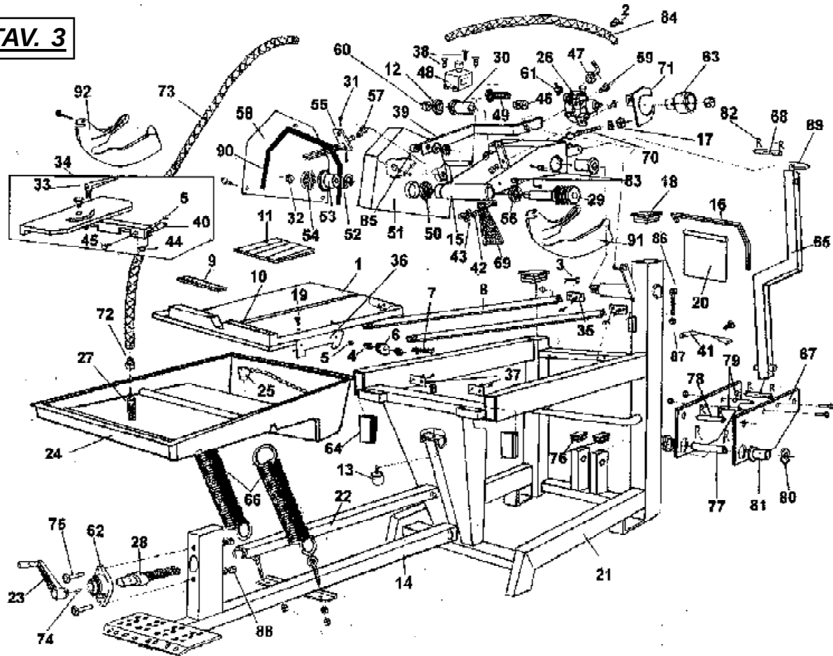
TAV.3 - MACHINE STRUCTURE
