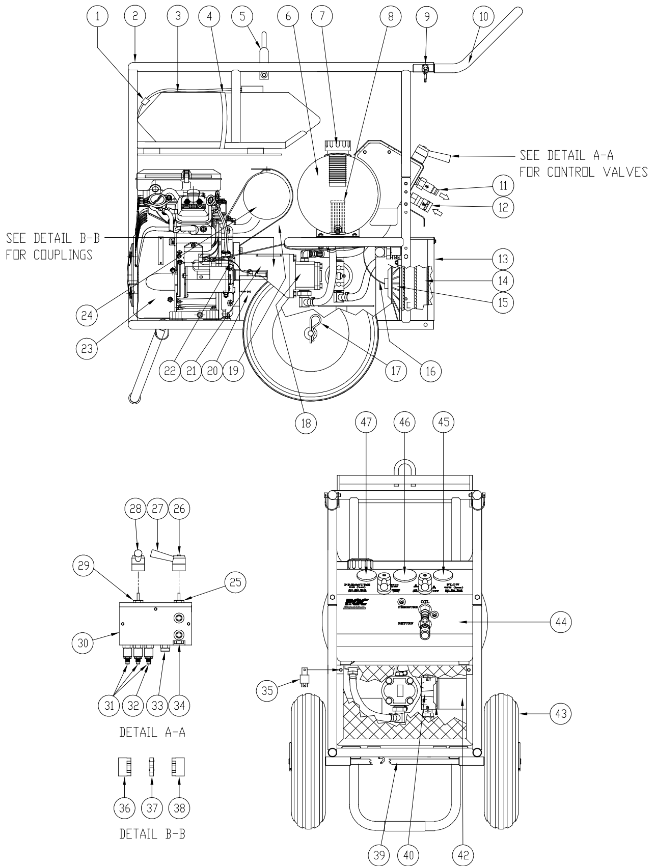
Figure 6-1. HH2210 & HH2212 Assembly Drawing
