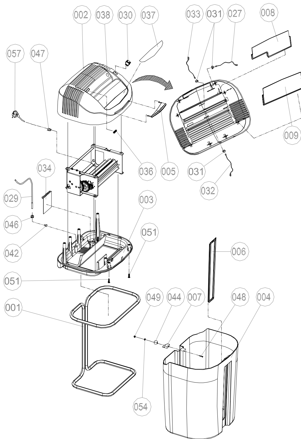
KOBRA +1 SS4/ +1SS6/ +1SS7 DISEGNO/DRAWING :01
