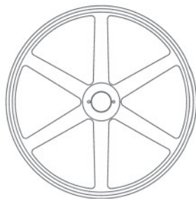
Part #0080 15" 2 groove Driven Pulley for Electric Powered Mixers
