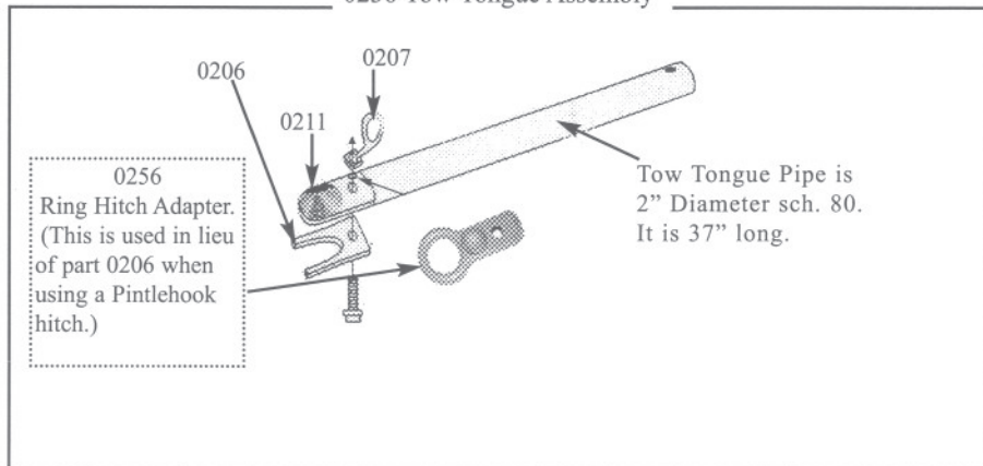
0236 Tow Tongue Assembly
