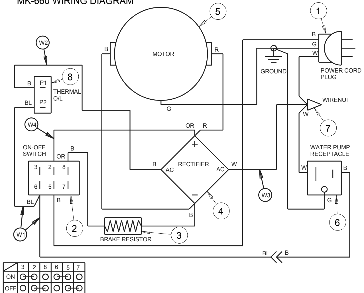
MK-660 WIRING DIAGRAM
