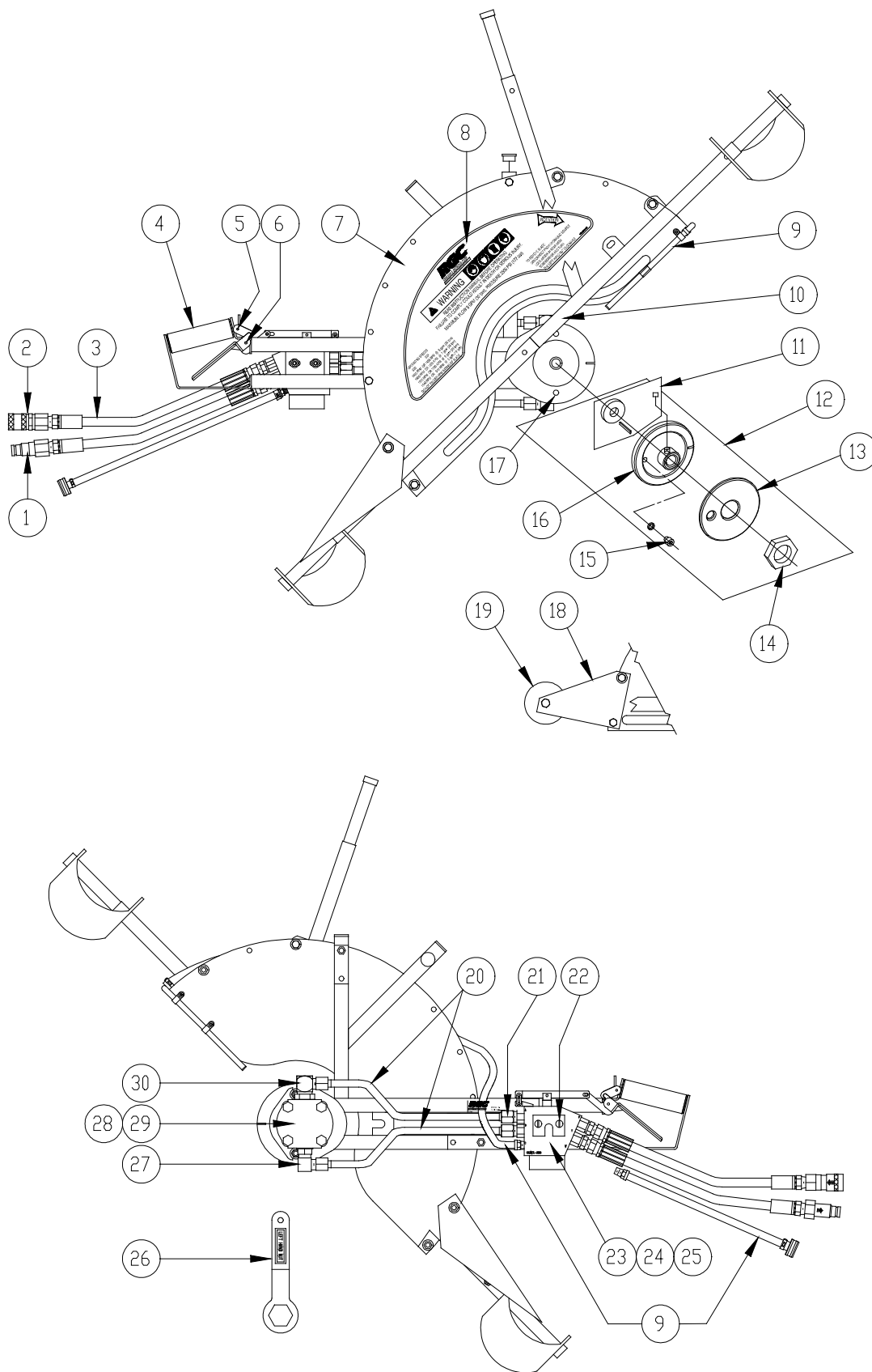
Figure 6-1. S20/S24 HydraSaw Assembly
