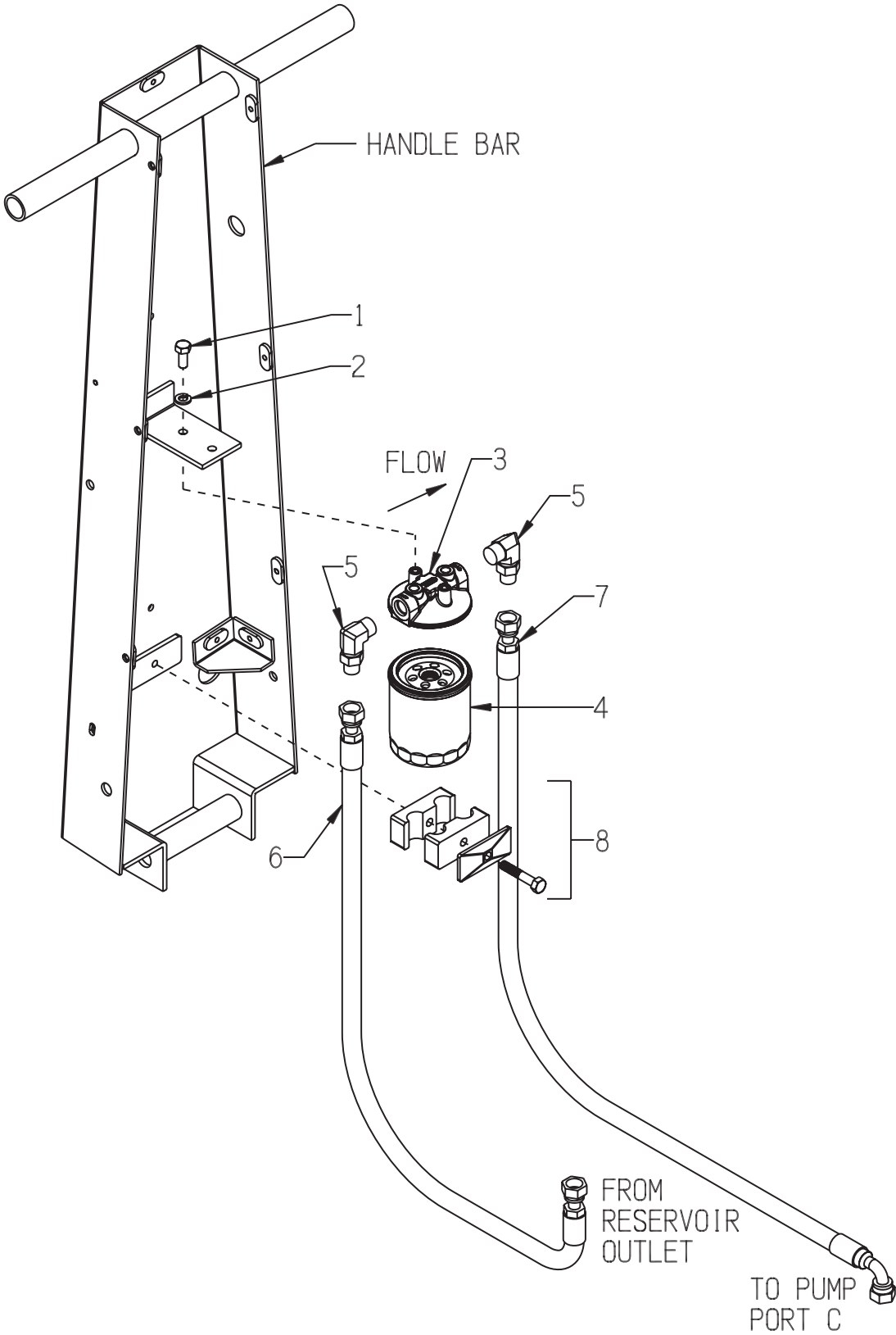
ILLUSTRATION 5 : FILTER GROUPING
