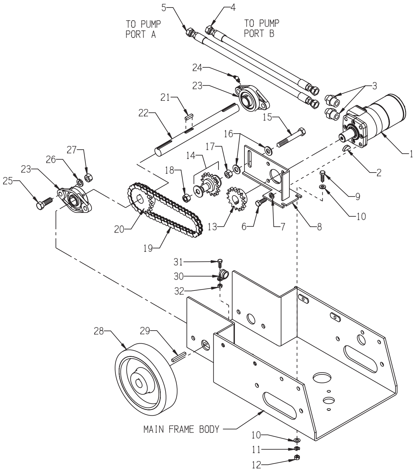
ILLUSTRATION 3 : DRIVE MOTOR & REAR AXLE GROUPING
