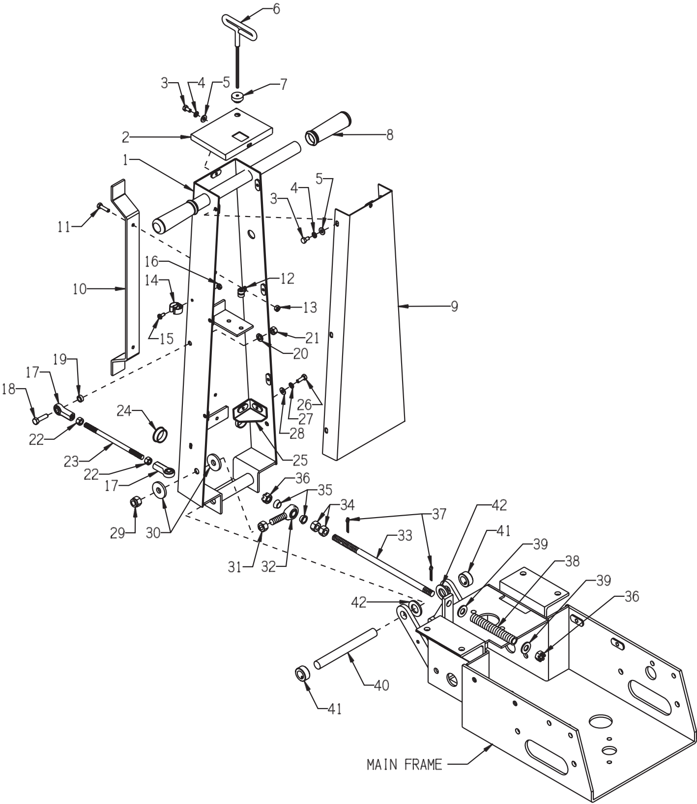
ILLUSTRATION 2 : HANDLE BAR GROUPING
