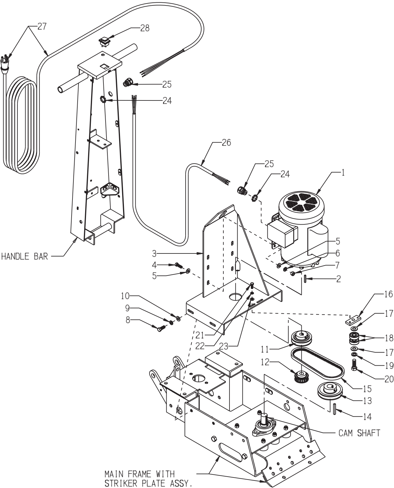
ILLUSTRATION 8 : MOTOR & BELT DRIVE GROUPING
