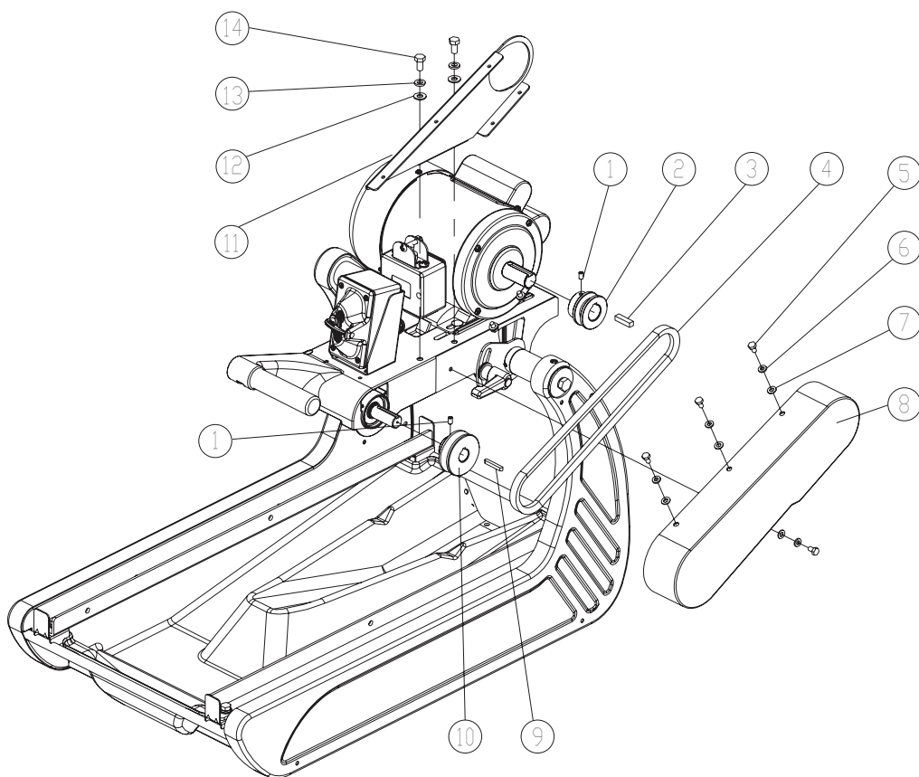
Belt Guard Assembly
