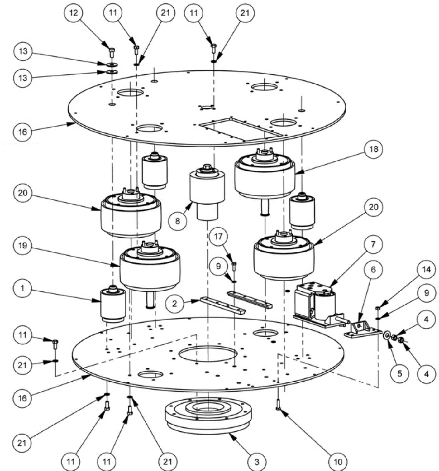
Fig. 9 - Drum Assembly
