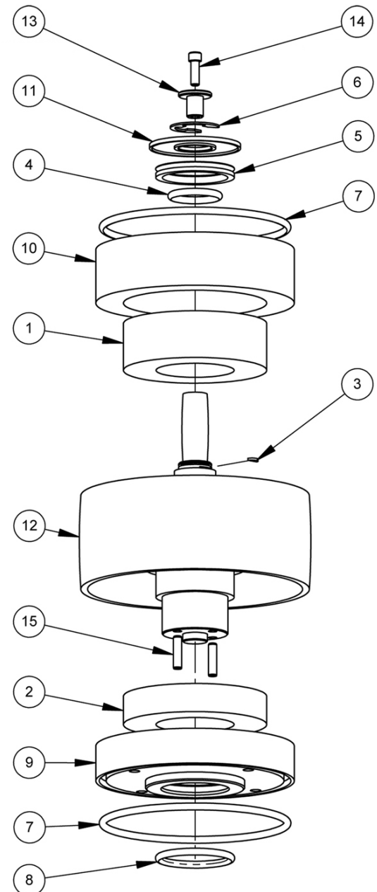
Fig. 14 - Cutter Head Assembly
