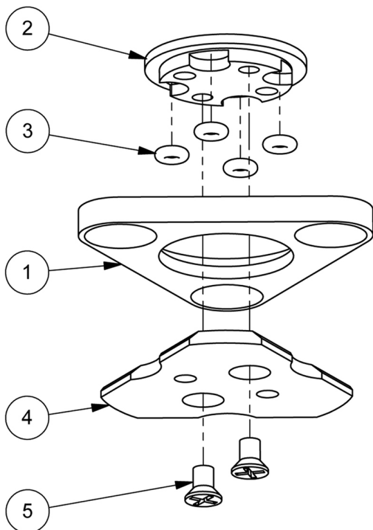
Fig. 18 - Holder Assembly
