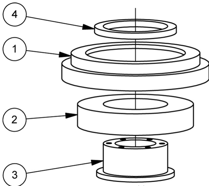
Fig. 11 - Bearing Assembly
