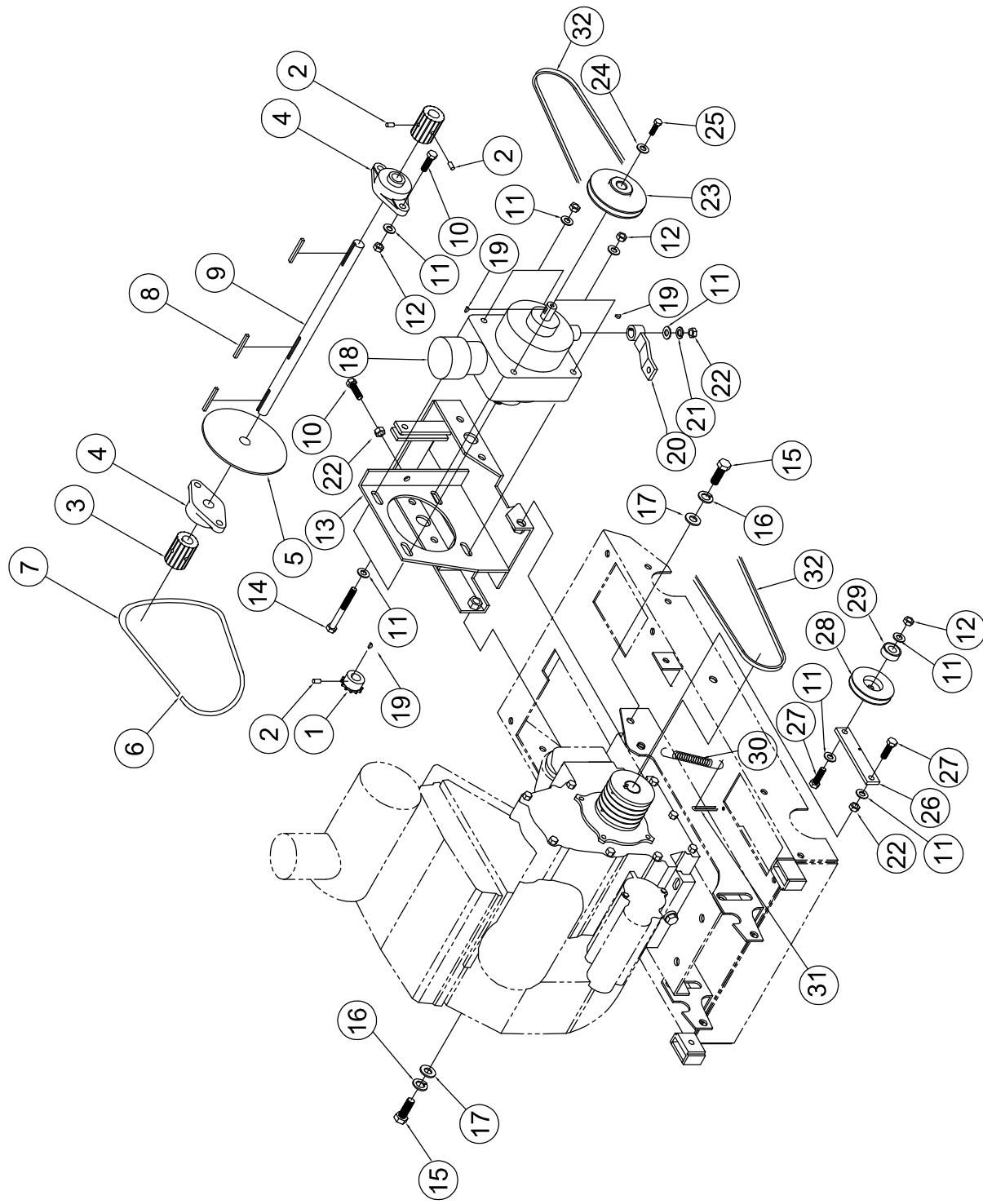
C13xxx ,C20xx, & PC20xx Transmission
