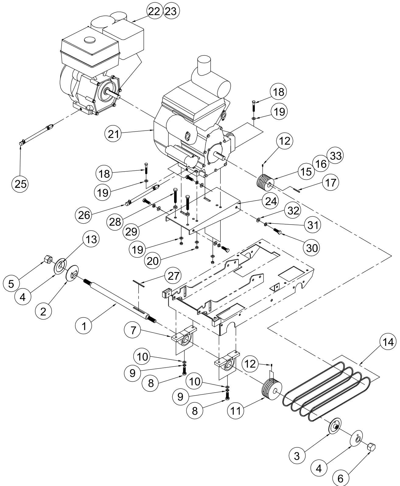
C13xxx ,C20xx, & PC20xx Blade Shaft & Engine Group
