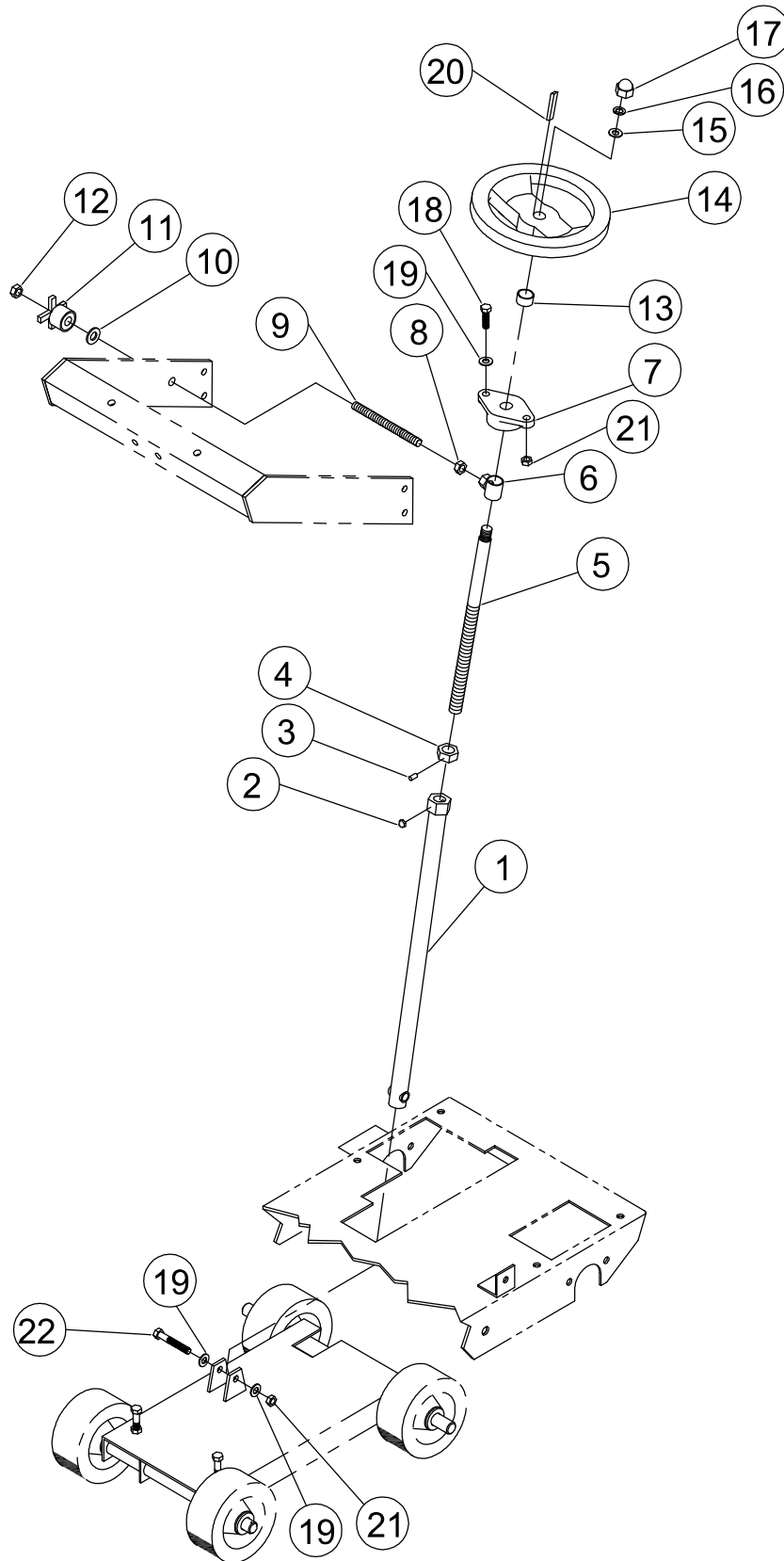
C13xxx ,C20xx, & PC20xx Depth Adjustment Group
