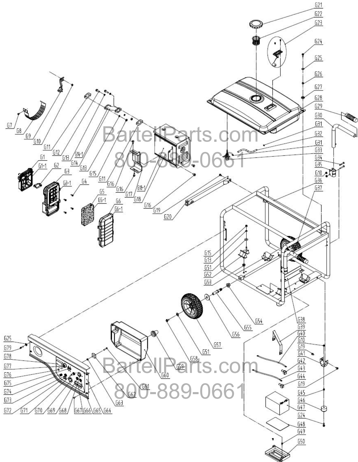
Frame, Control Panel, Muffler, Fuel Tank and Air Cleaner: BG7500E – Parts List 4
