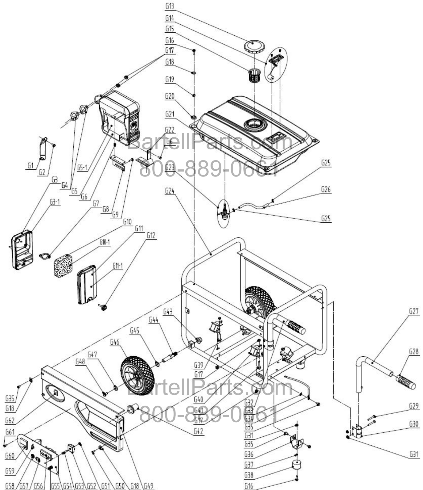
Frame, Control Panel, Muffler, Fuel Tank and Air Cleaner: BG2800 – Parts List 2
