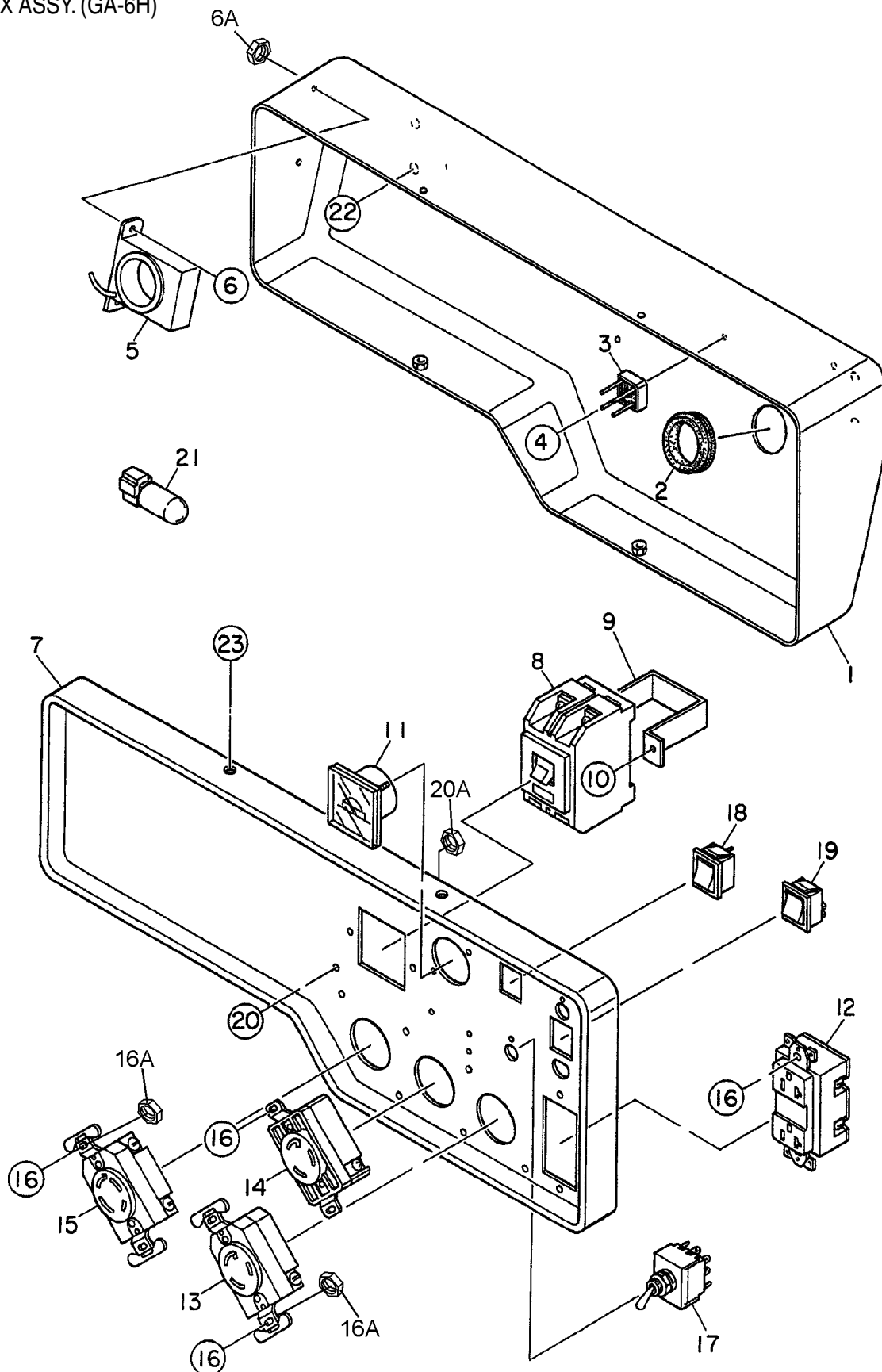
CONTROL BOX ASSY. (GA-6H)
