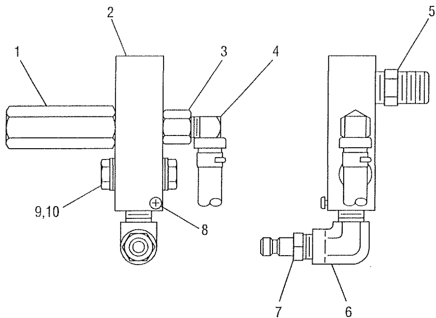
Figure 20 - Coil Outlet Assembly
