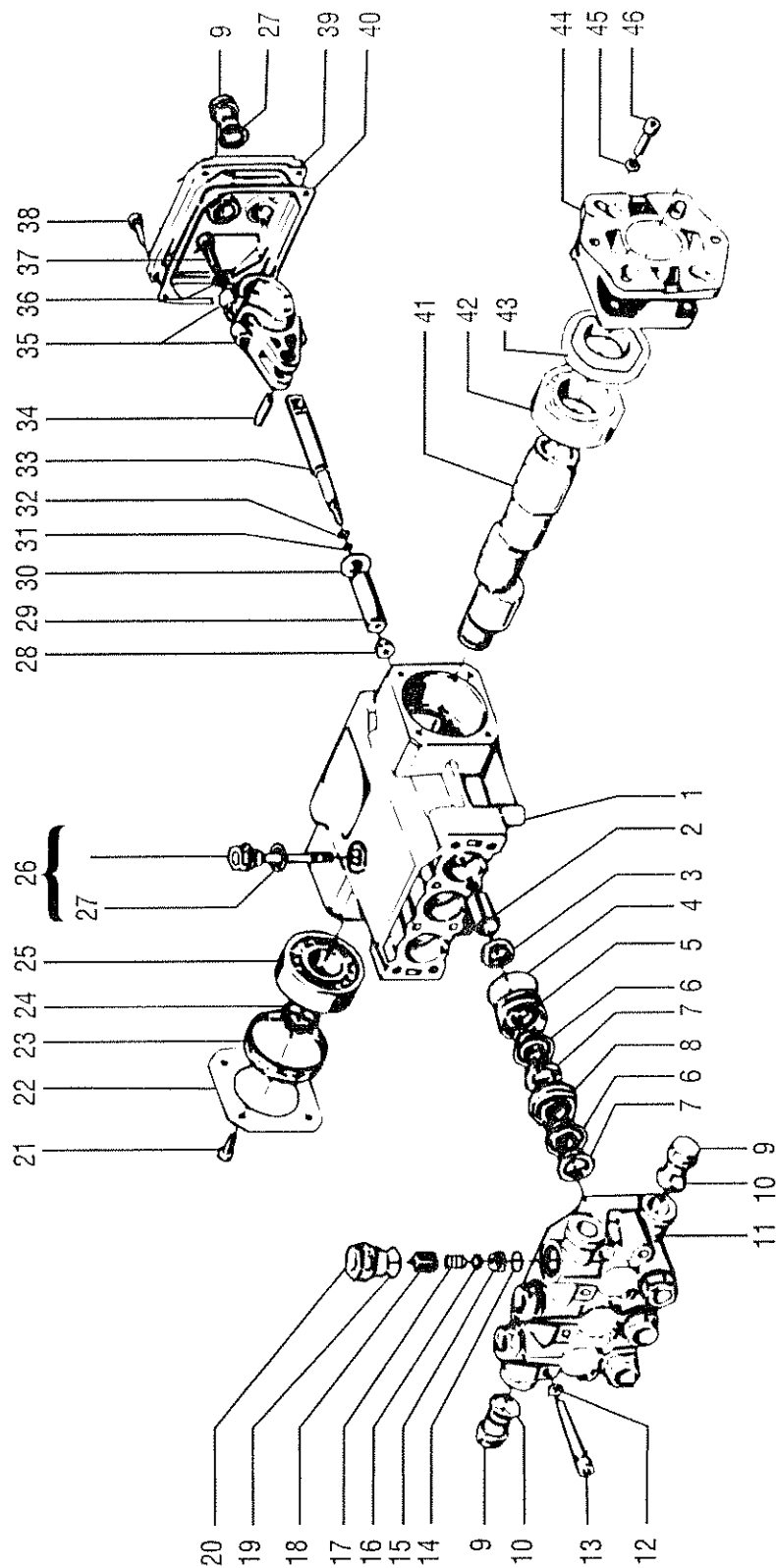
Figure 16 - Pump, Exploded View
