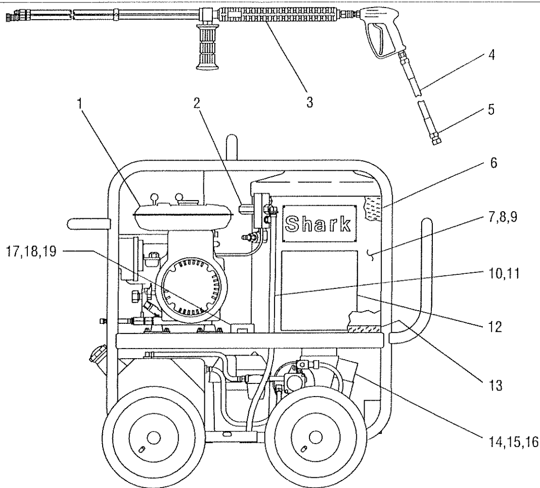
Figure 12 - Machine Assembly, Right Side View
