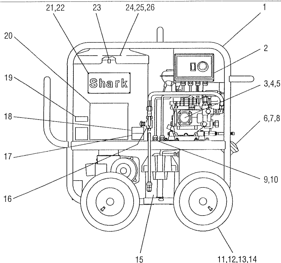
Figure 11 - Machine Assembly, Left Side View
