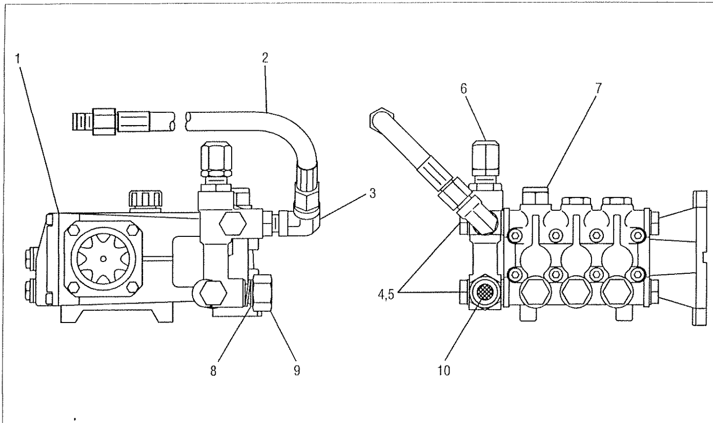
Figure 15 - Pump Assembly
