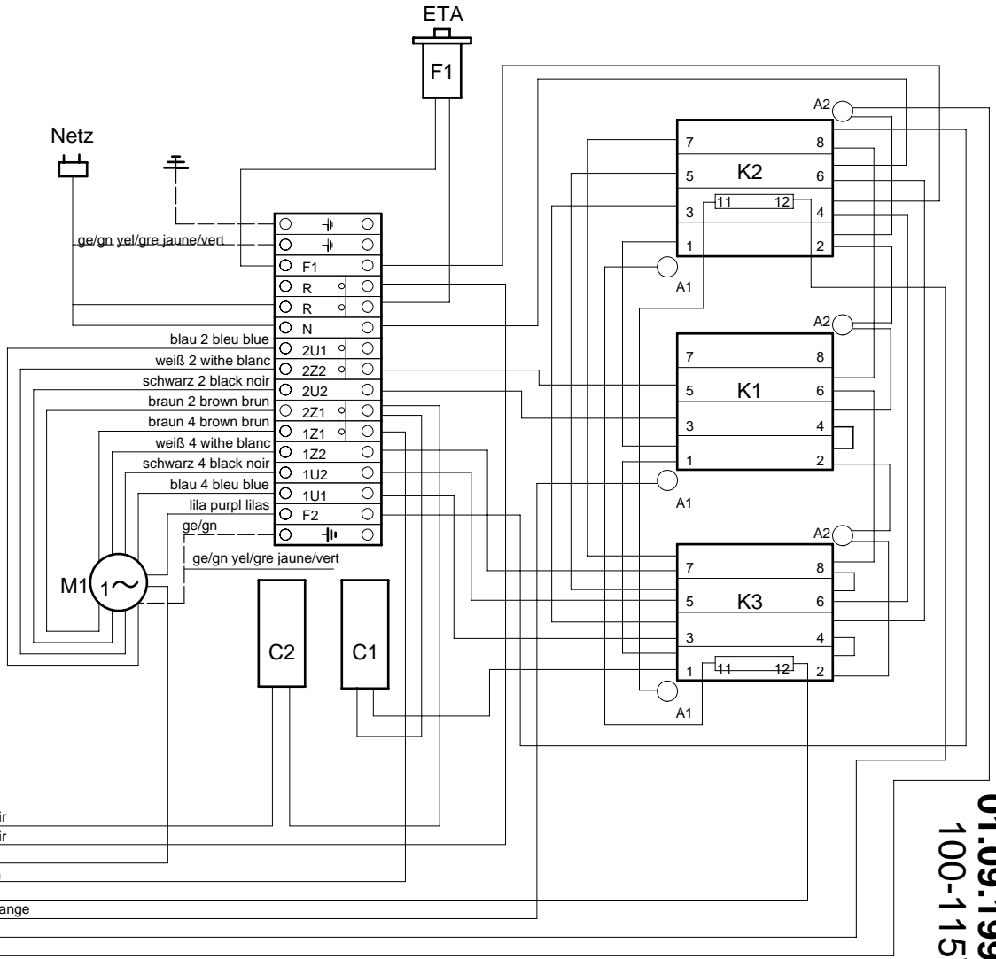
Anschlußplan 4004 E CROSS/CUT Diagramme de branchement 4004 E CROSS/CUT Conecting diagram 4004 E CROSS/CUT
