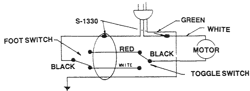
WIRING DIAGRAM
