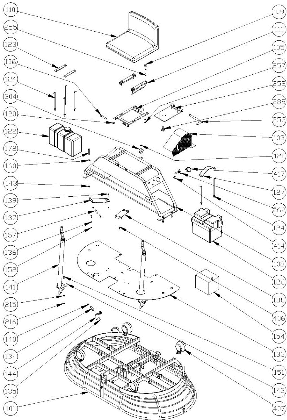
Figure 1 - Complete Chassis
