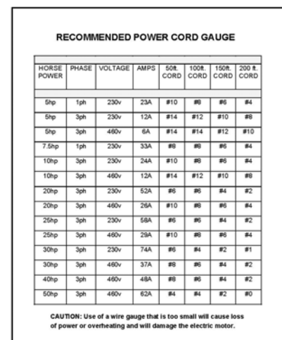
POWER CORD DECAL #1800376
