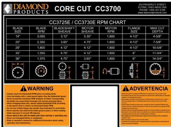
RPM CHART DECAL #1800582
