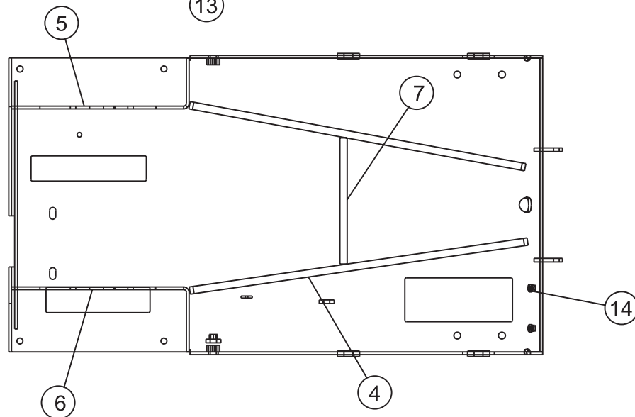
BOTTOM VIEW
