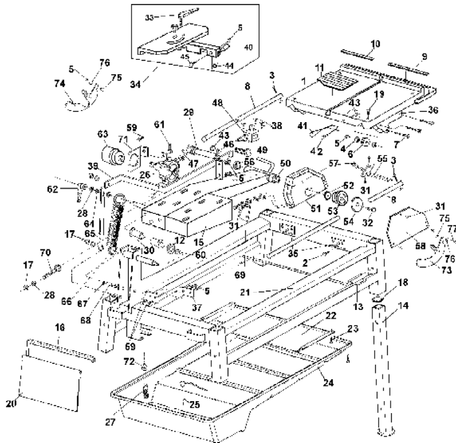
TAV. 4 - MACHINE STRUCTURE
