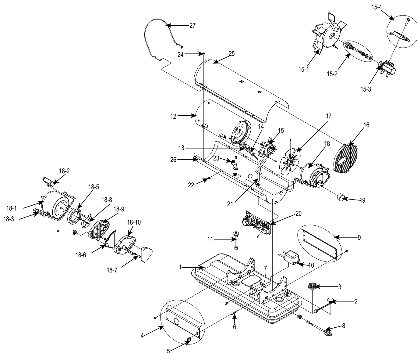
Figure 24– Repair Parts Illustration for Portable Oil-Fired Heaters Models CP045CK, CP075CK
