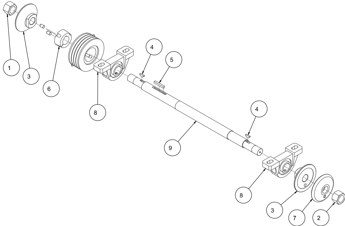
FIGURE 10 - BLADE SHAFT - P/N 170864
