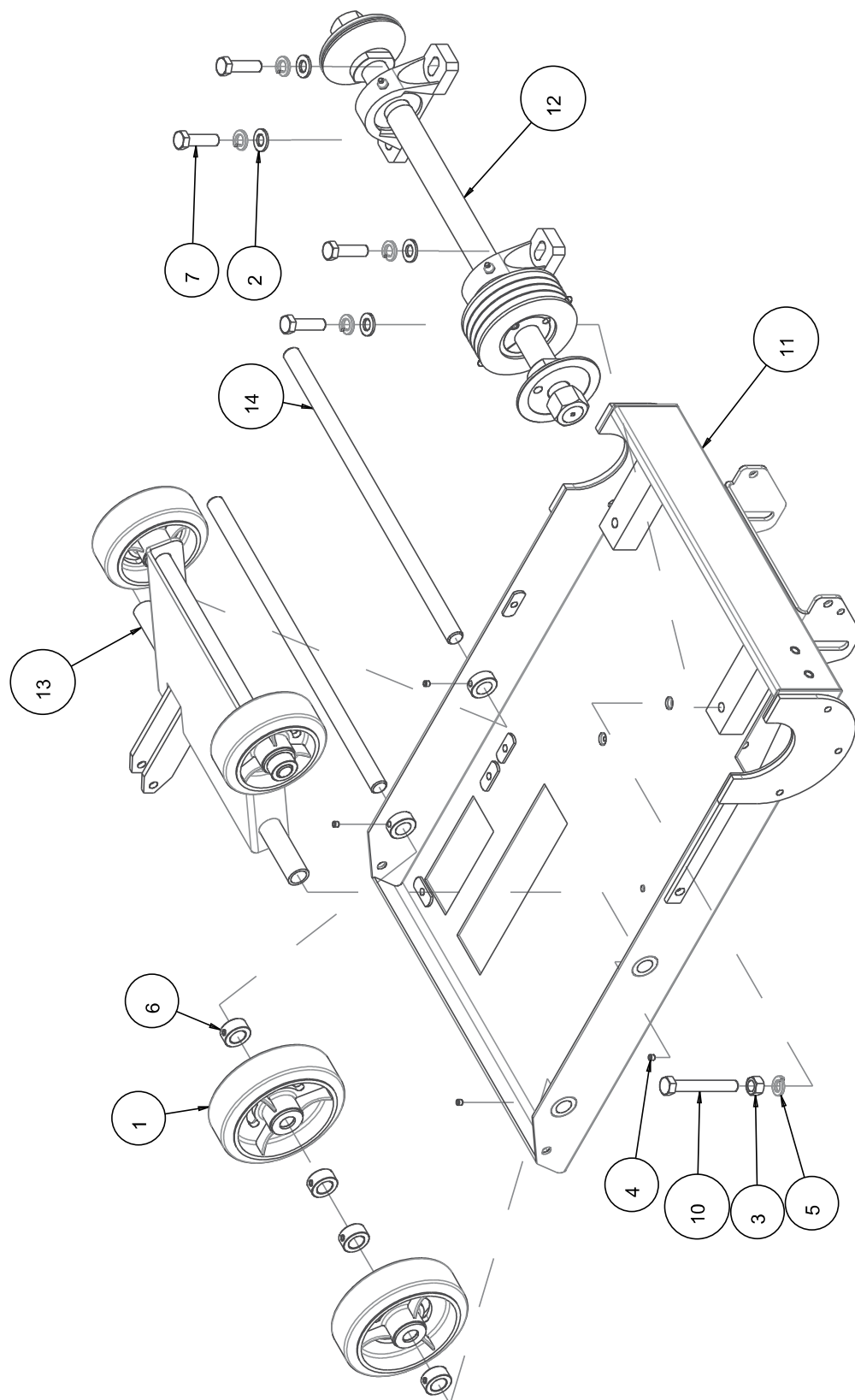
FIGURE 4 - FRAME, LESS ENGINE - P/N 170870-H
