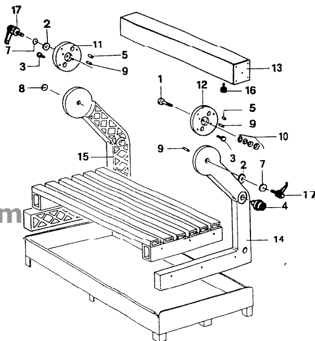
DIAG LOC. PART NO. DESCRIPTION 1 174064 Bolt 2 174131 Washer 3 174101 Screw 4 174254 Knob 5 174113 Spacer 6 174119 Nut 7 174124 Washer 8 174131 Washer 9 174144 Locating Pin 10 174149 Spring 11 174155 Location Disc 12 174156 Location Disc 13 174203 Travel Column 14 174184 Support Arm 15 174185 Support Arm 16 174215 Shock Absorber 17 174230 Handle
