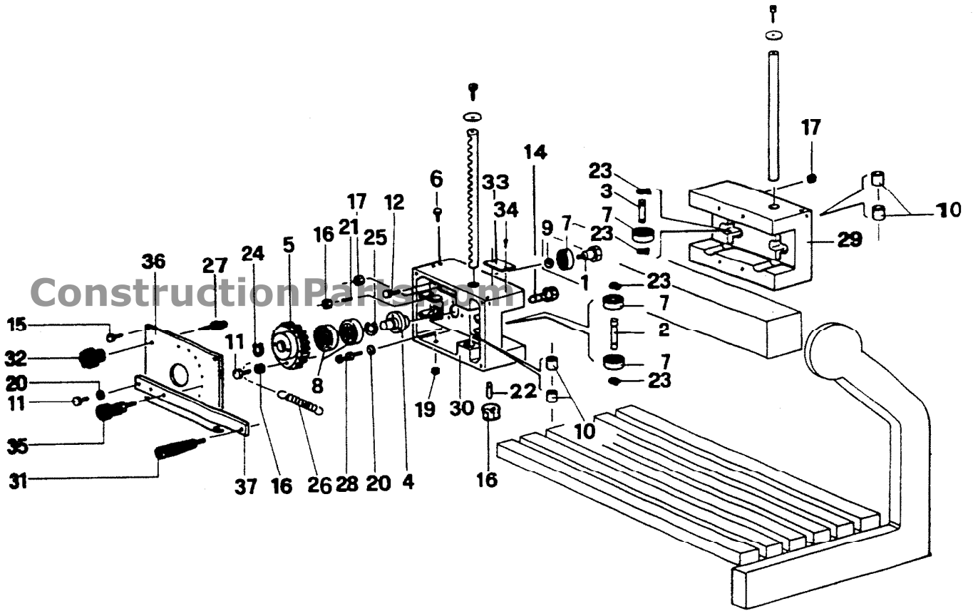
FIGURE 3 - ASSEMBLY OF CARRIAGE PARTS LIST
