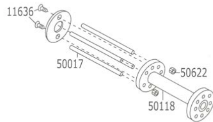
"B" CAGE ASSEMBLY - 50146
