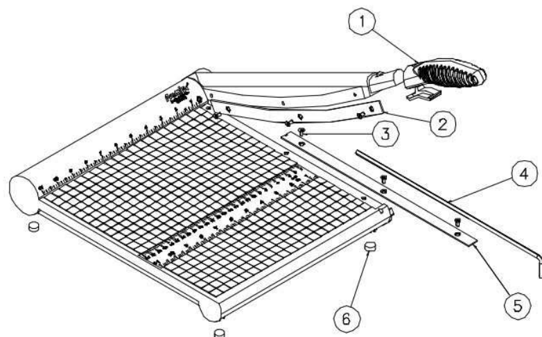
P212X PARTS LIST
