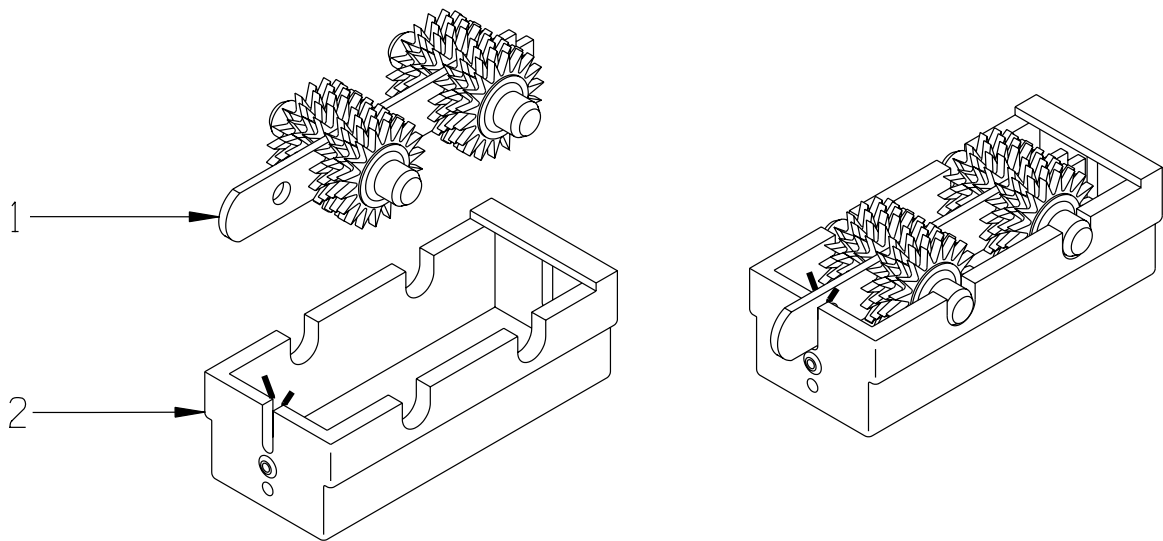
ILLUSTRATION 15 : SCARIFIER ACCESSORY
