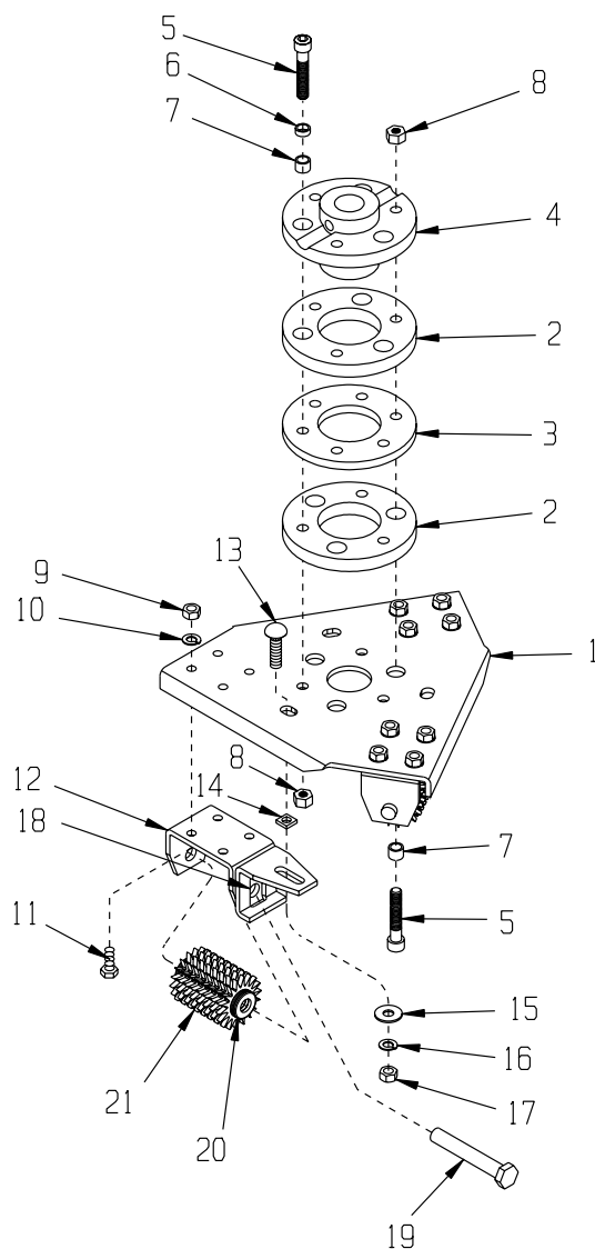
ILLUSTRATION 4 : OPTIONAL SURFACER DISC ASSEMBLY
