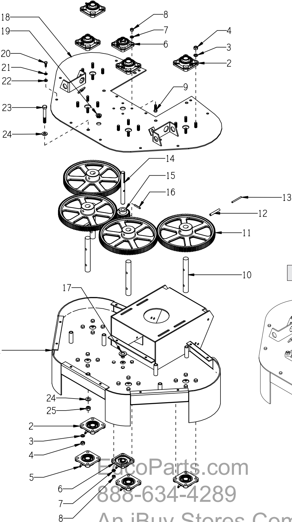
ILLUSTRATION 1 : GEAR CASE ASSEMBLY
