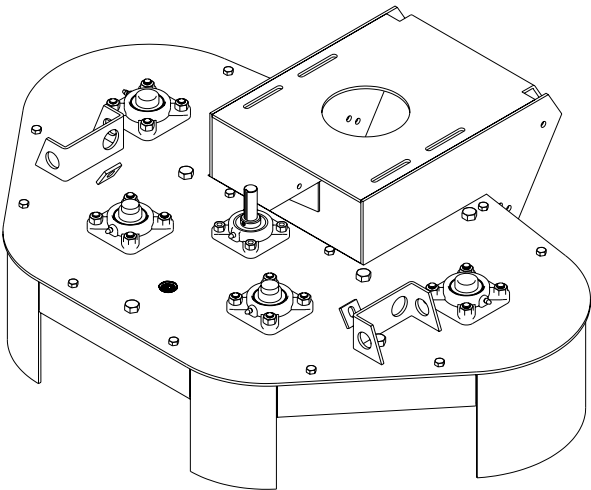
GEAR CASE ASSEMBLED
