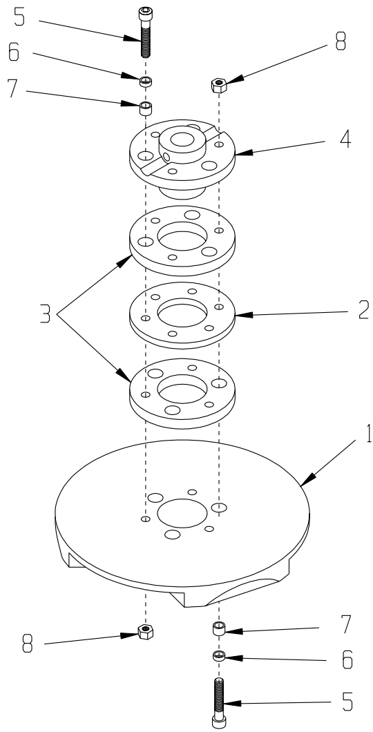
ILLUSTRATION 2 : MULTI-ACCESSORY DISC ASSEMBLY
