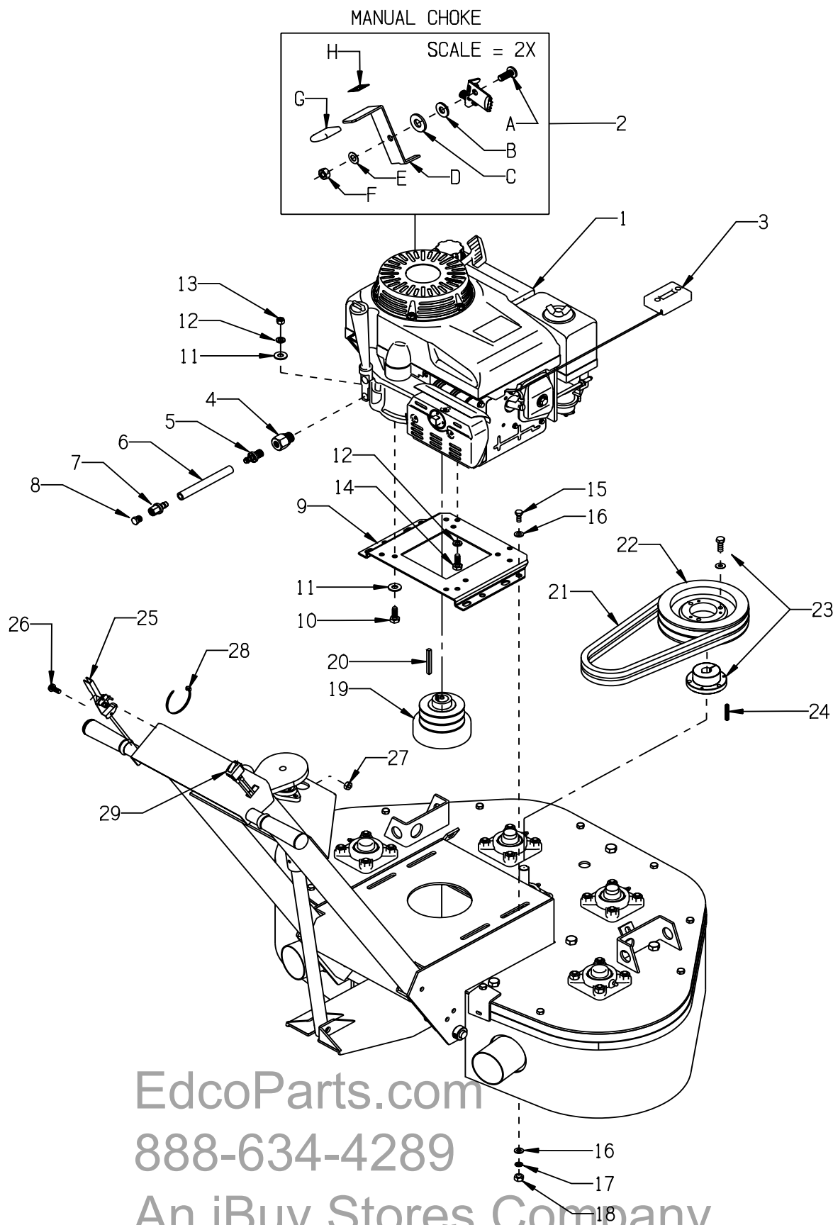
ILLUSTRATION 9: ENGINE & BELT DRIVE GROUPING
