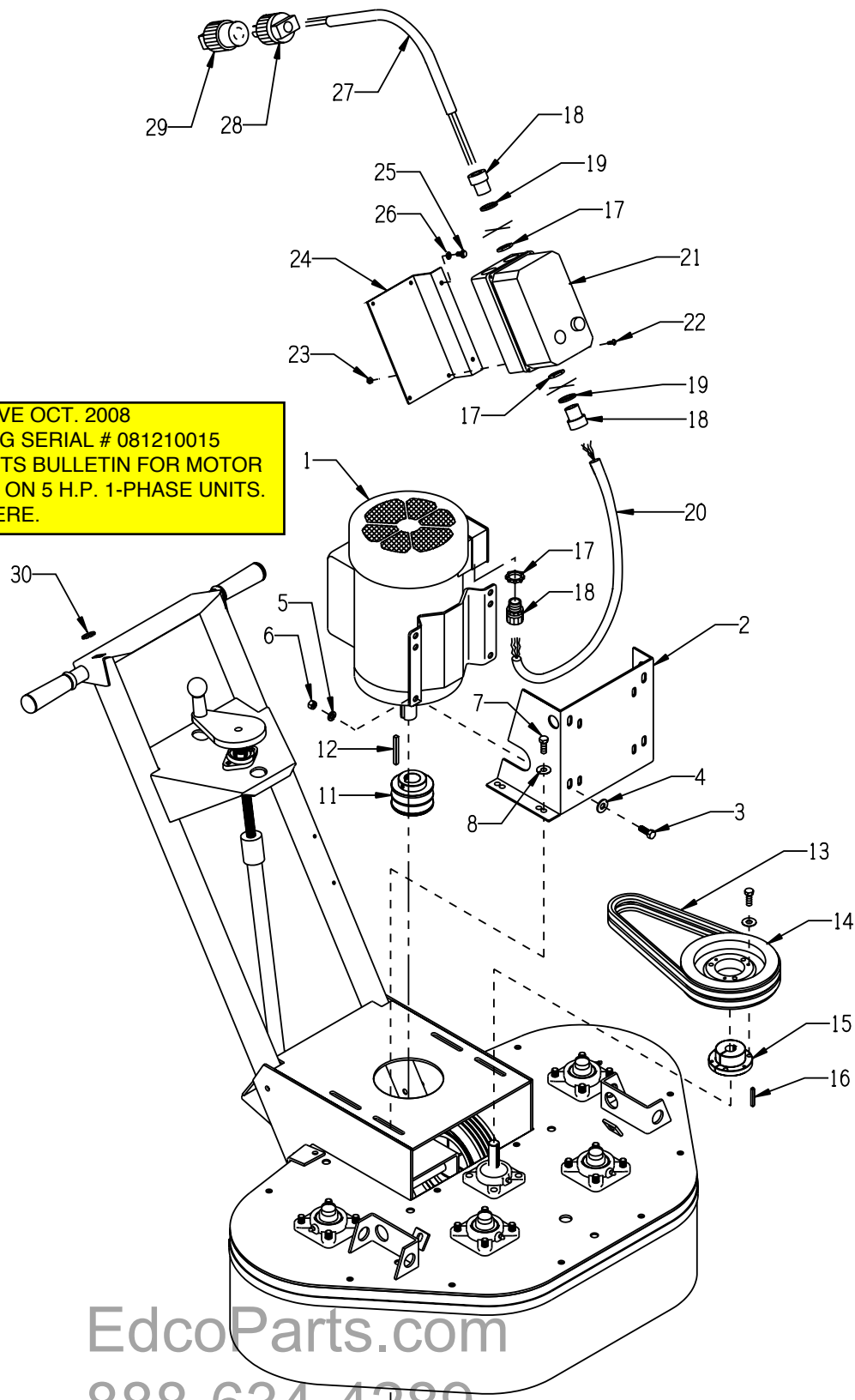
ILLUSTRATION 11: MOTOR & BELT DRIVE GROUPING
