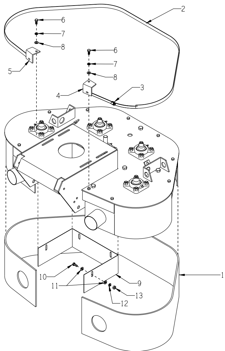
ILLUSTRATION 7: SKIRT GROUPING
