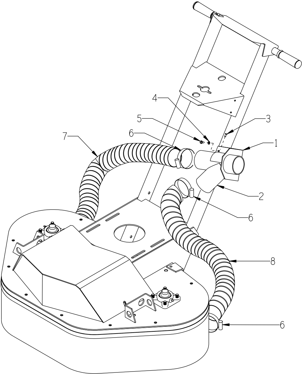
ILLUSTRATION 8 : VACUUM PORT & HOSE GROUPING
