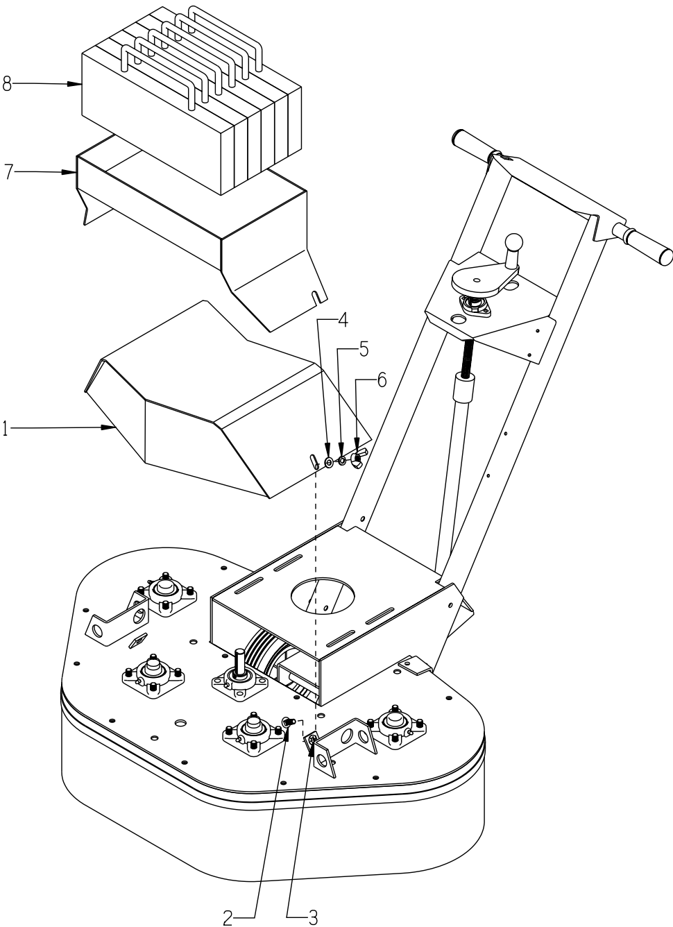
ILLUSTRATION 12 : HOOD, OPTIONAL WEIGHT TRAY & WEIGHT BLOCKS
