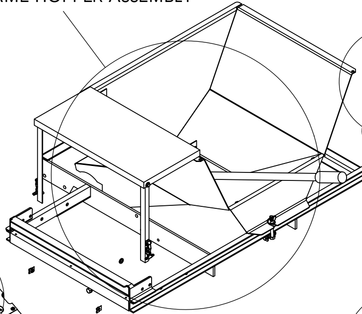
FRAME-HOPPER ASSEMBLY
