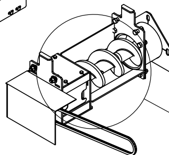
AUGER ASSEMBLY
