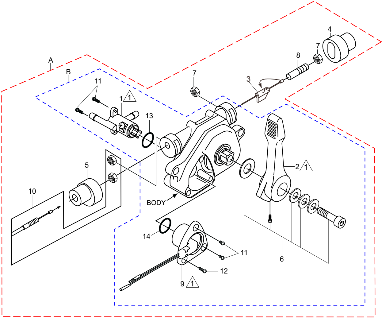
DETAIL C
