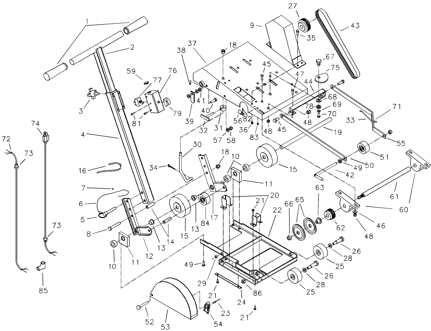
FIGURE 1 - EXPLODED VIEW (ALL MODELS)
