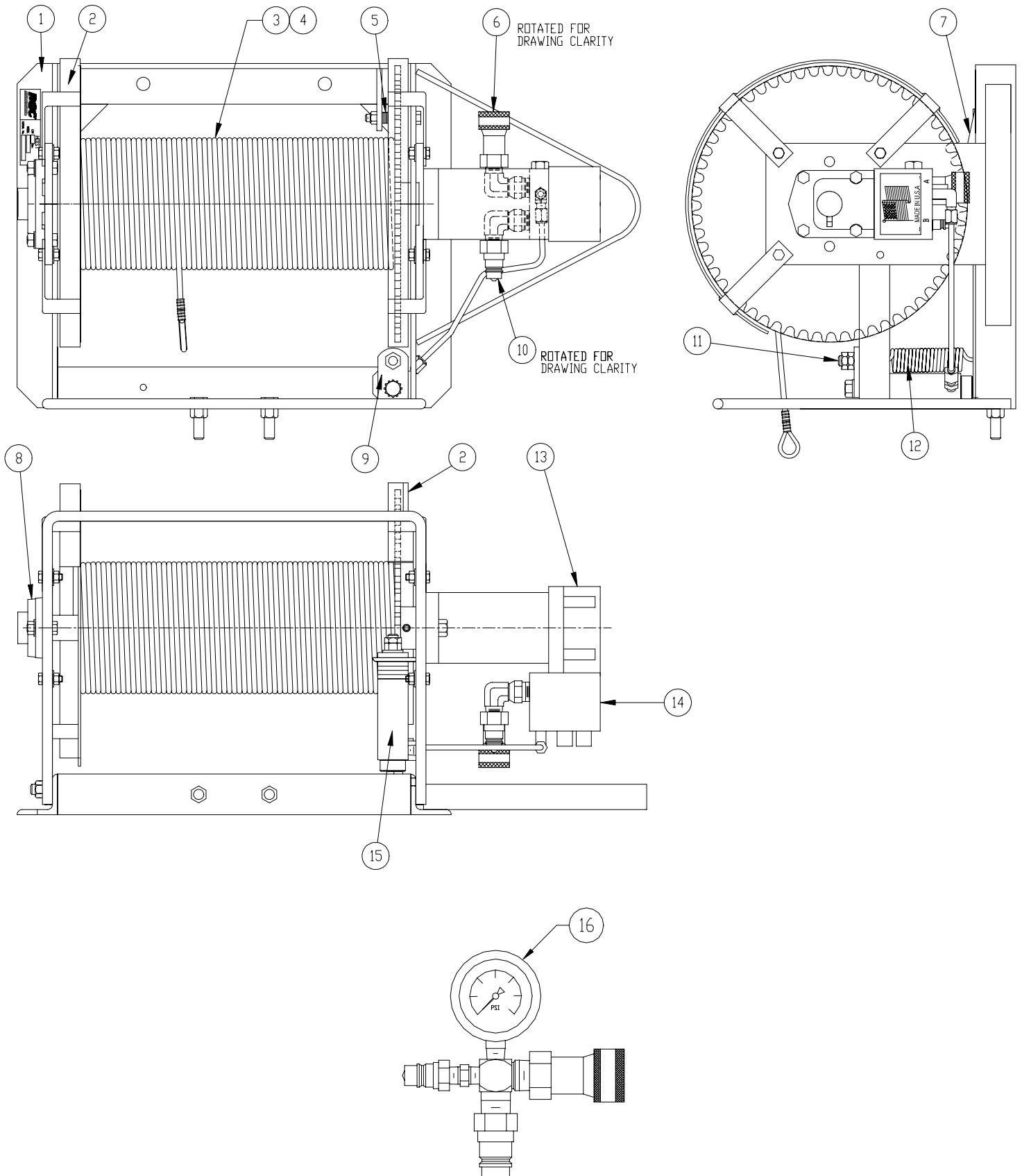
Figure 8-1. HydraWinch HD Assembly Drawing
