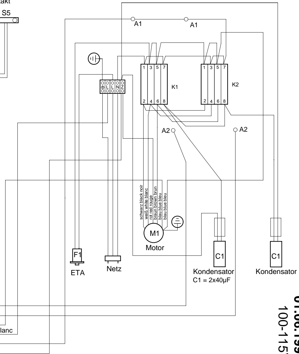
Anschlußplan 4000 E CROSS/CUT Diagramme de branchement 4000 E CROSS/CUT Conecting diagram 4000 E CROSS/CUT
