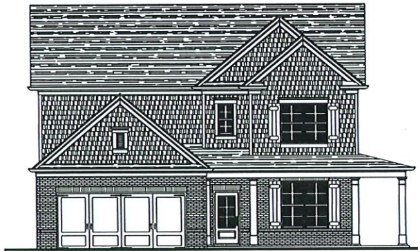
Front Elevation C
