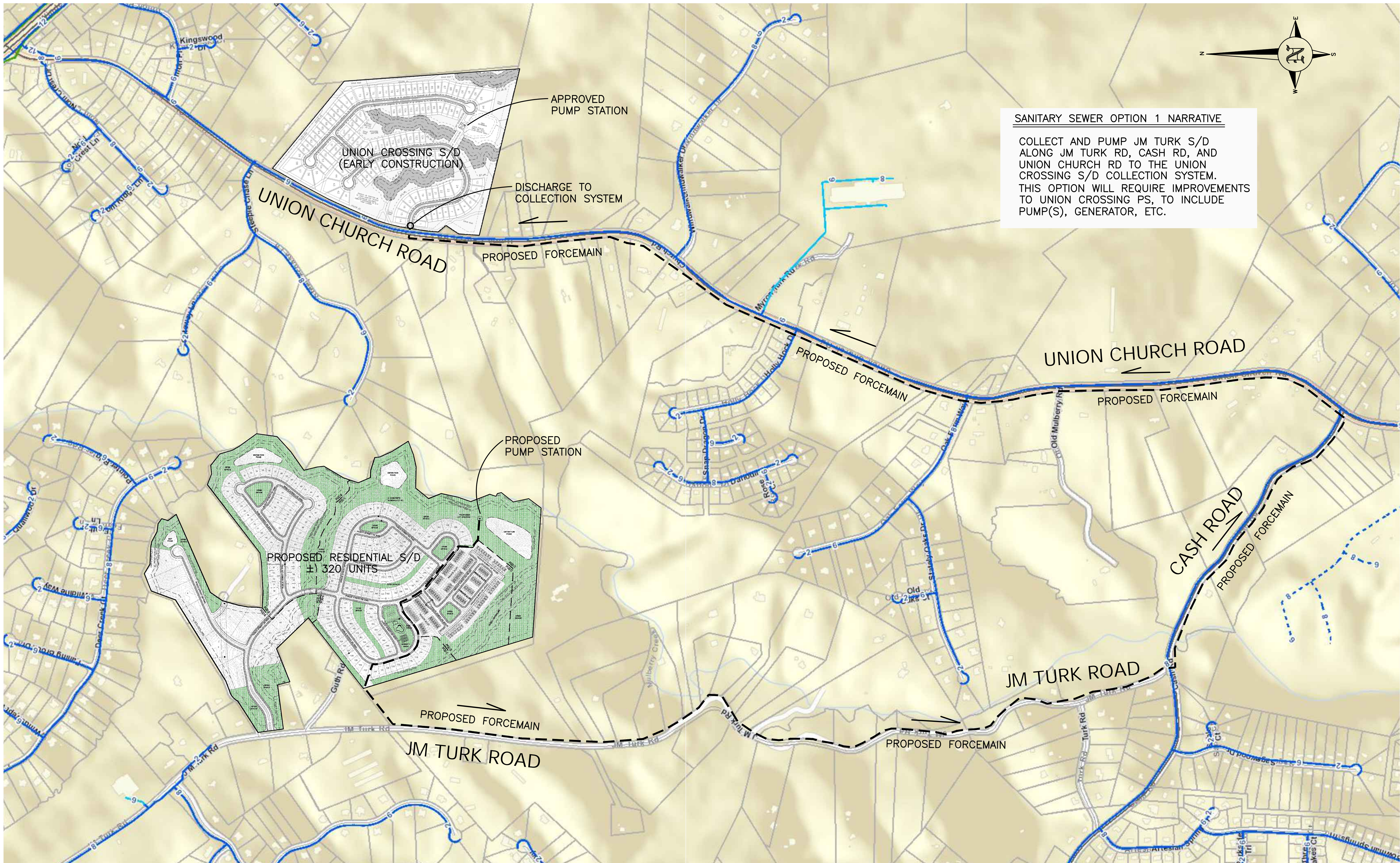
SANITARY SEWER CONCEPT PLAN SCALE: 1" = 400'
