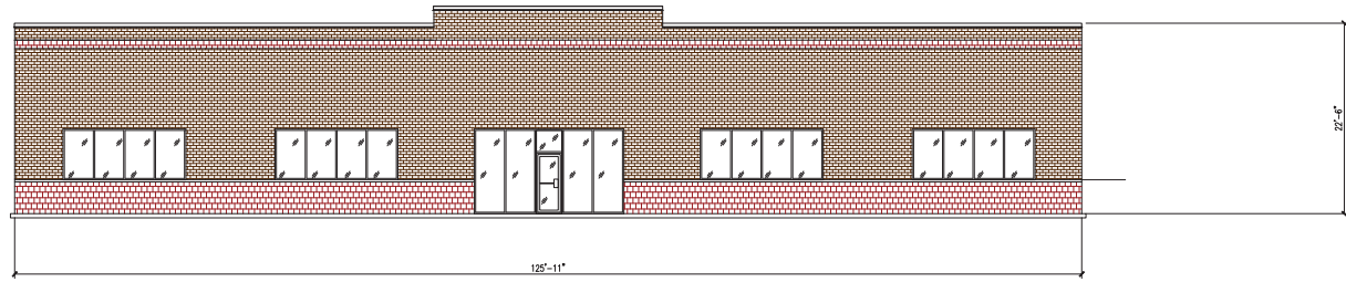
FRONT ELEVATION
