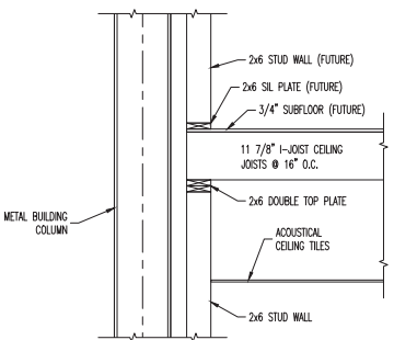
2 CEILING FRAMING DETAIL S3 SCALE: 3/4"=1'-0"
