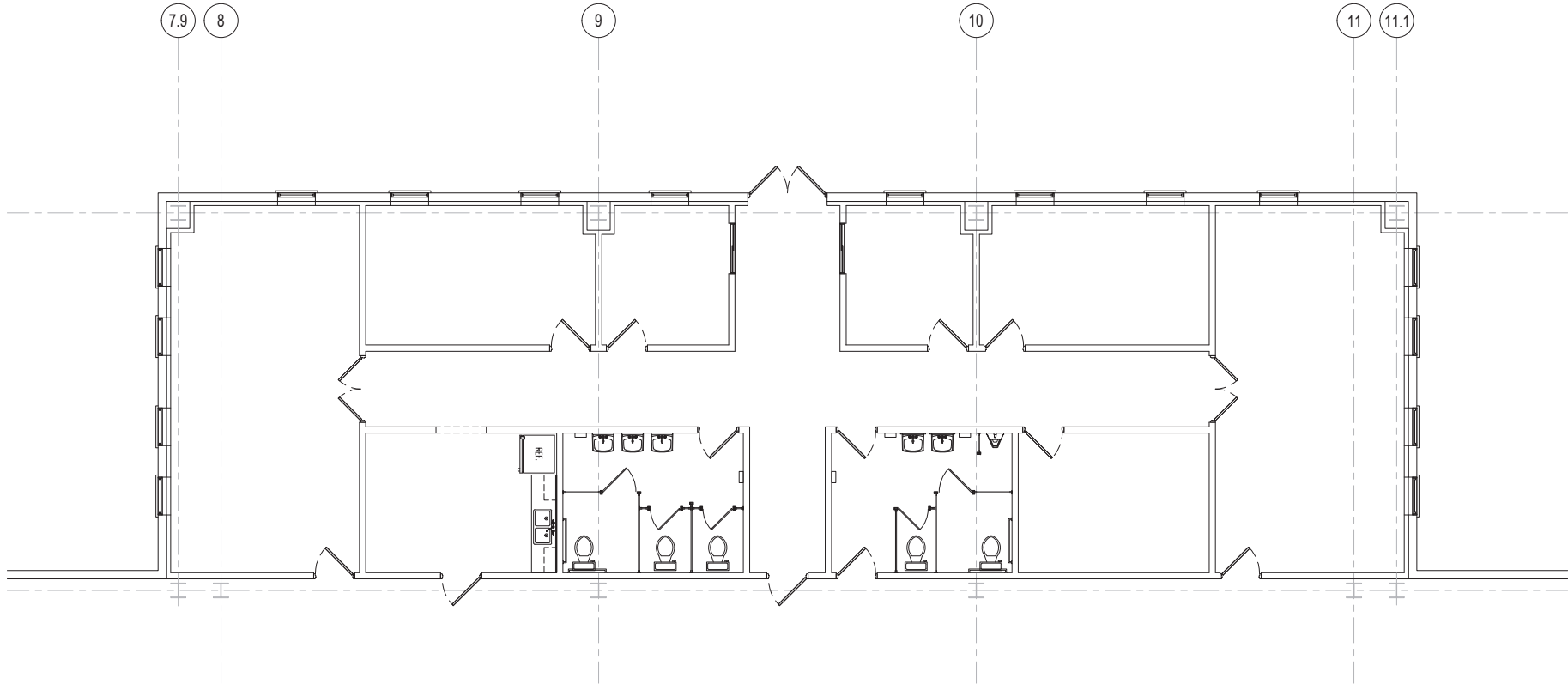
1 PLUMBING PLAN - WASTE WATER (OFFICE) P4 SCALE: 1/4"=1'-0"
