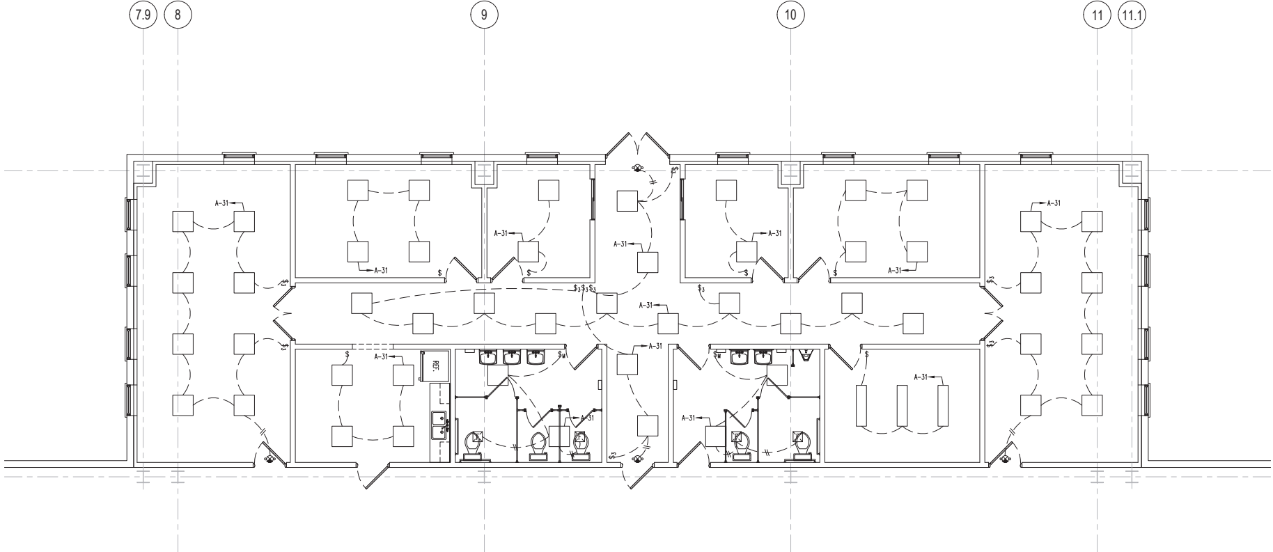
1 LIGHTING PLAN (OFFICE) E2 SCALE: 1/4"=1'-0"
