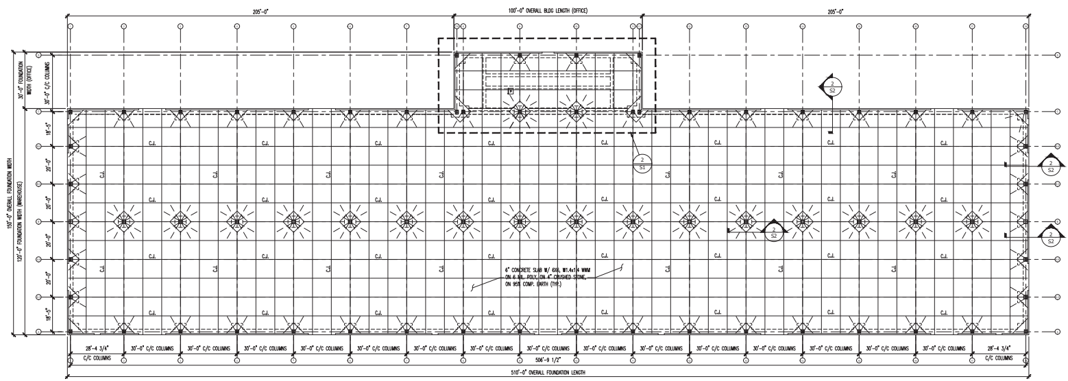
1 FOUNDATION PLAN S1 SCALE: 1/16"=1'-0"
