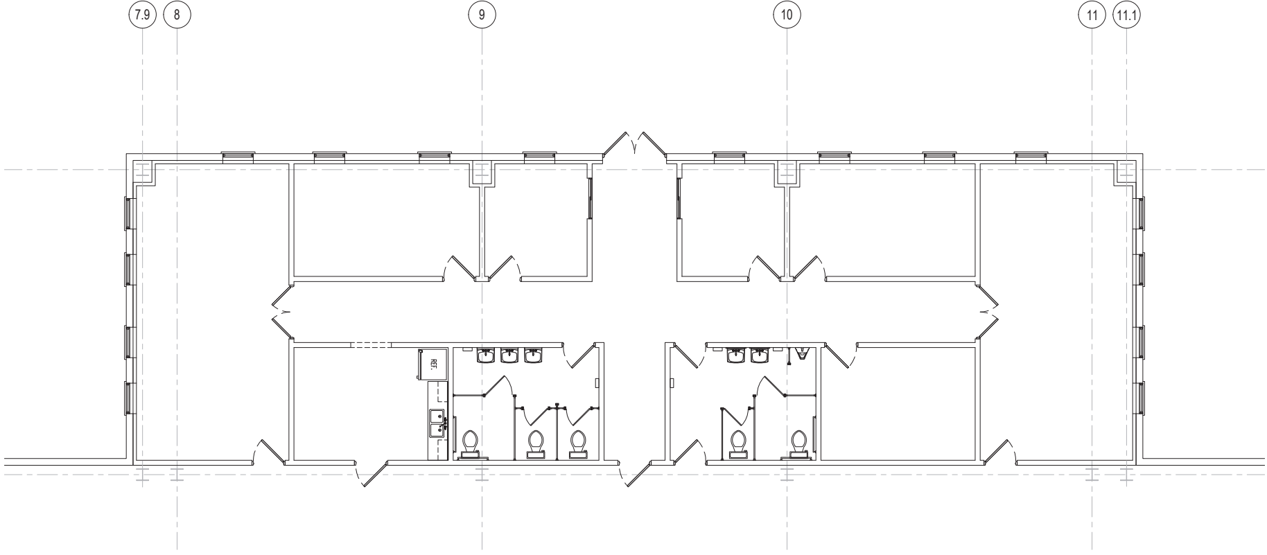
1 POWER PLAN (OFFICE) E3 SCALE: 1/4"=1'-0"
