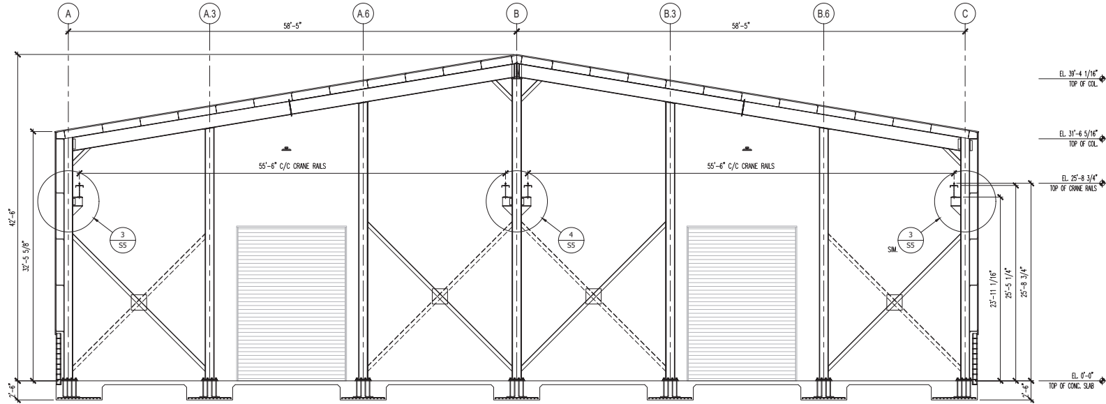
1 BUILDING CROSS SECTION (WAREHOUSE) A5 SCALE: 3/16"=1'-0"
