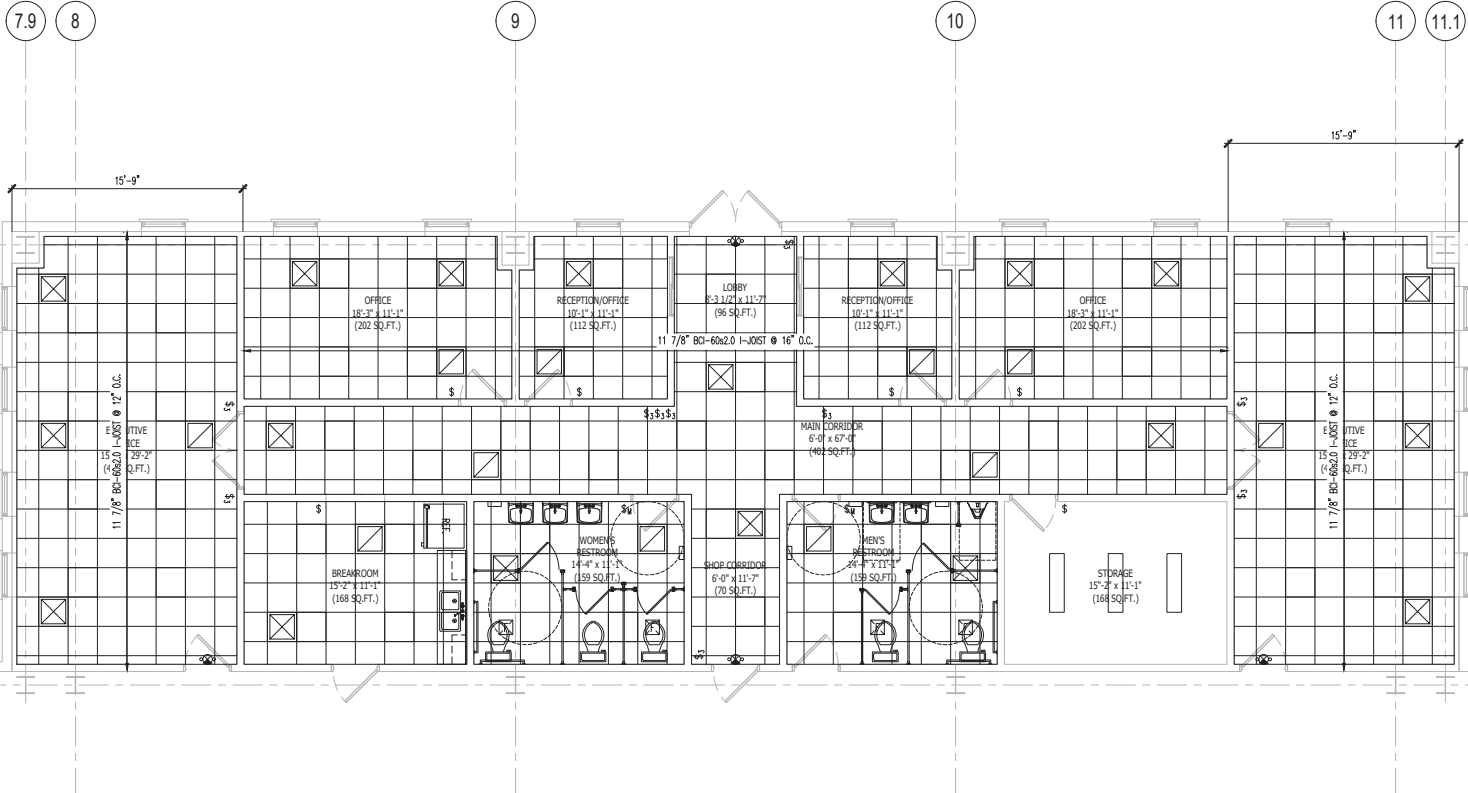
1 REFLECTED CEILING PLAN (OFFICE) A6 SCALE: 1/4"=1'-0"
