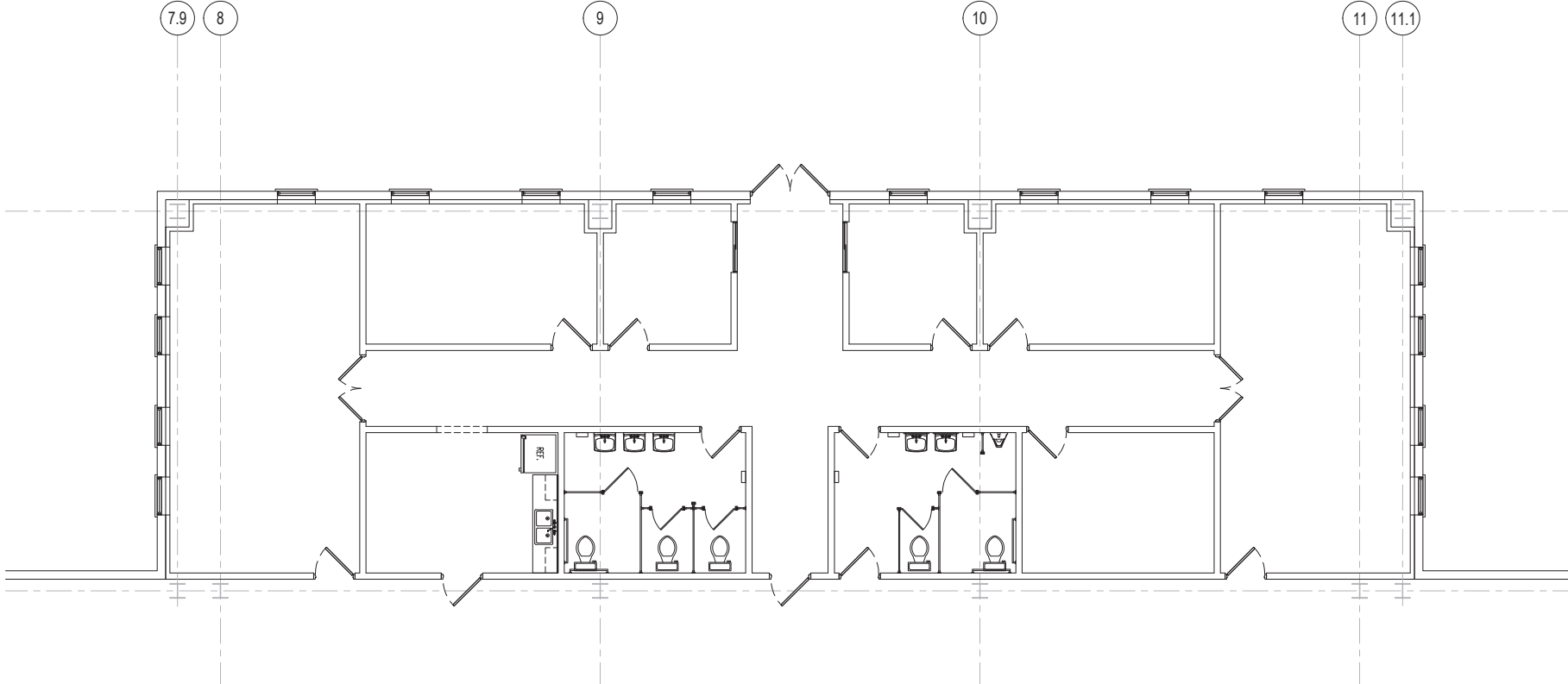
1 PLUMBING PLAN - SUPPLY (OFFICE) P2 SCALE: 1/4"=1'-0"
