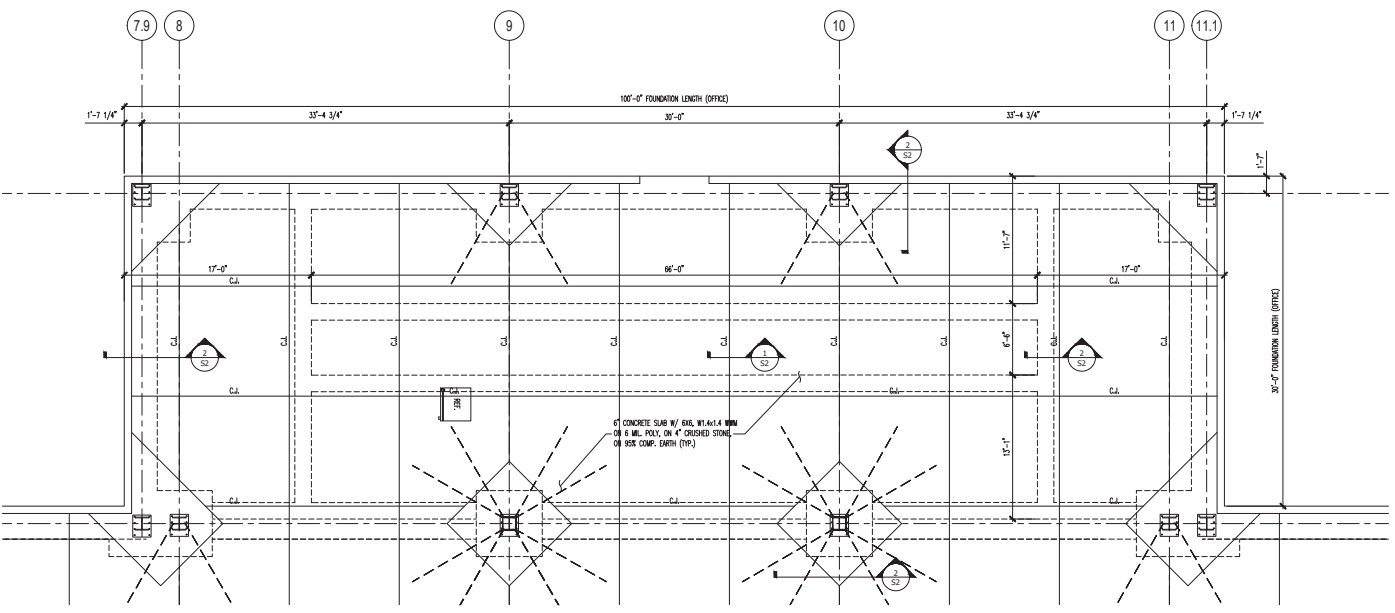
2 ENLARGED VIEW FOUNDATION PLAN (OFFICE) S1 SCALE: 1/4"=1'-0"
