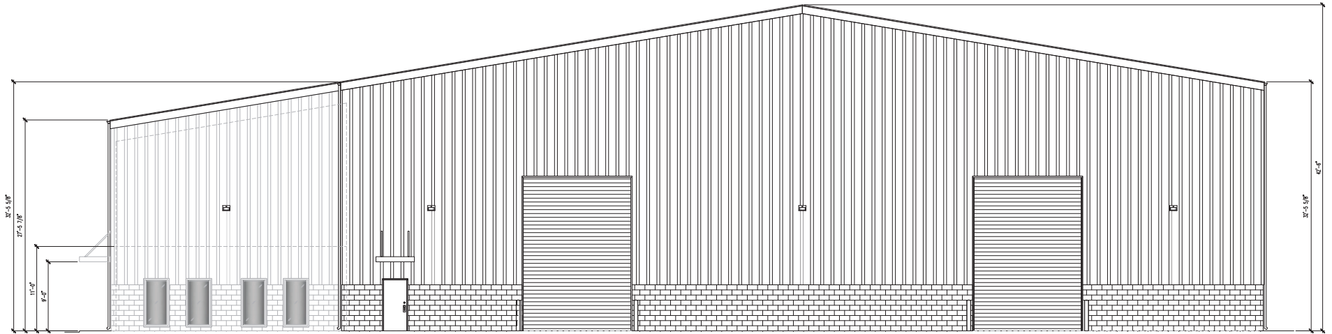
RIGHT ELEVATION SCALE: 3/16"=1'-0"
