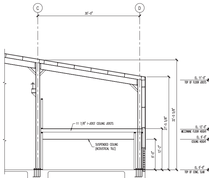
1 BUILDING CROSS SECTION (WAREHOUSE) A5 SCALE: 3/16"=1'-0"
