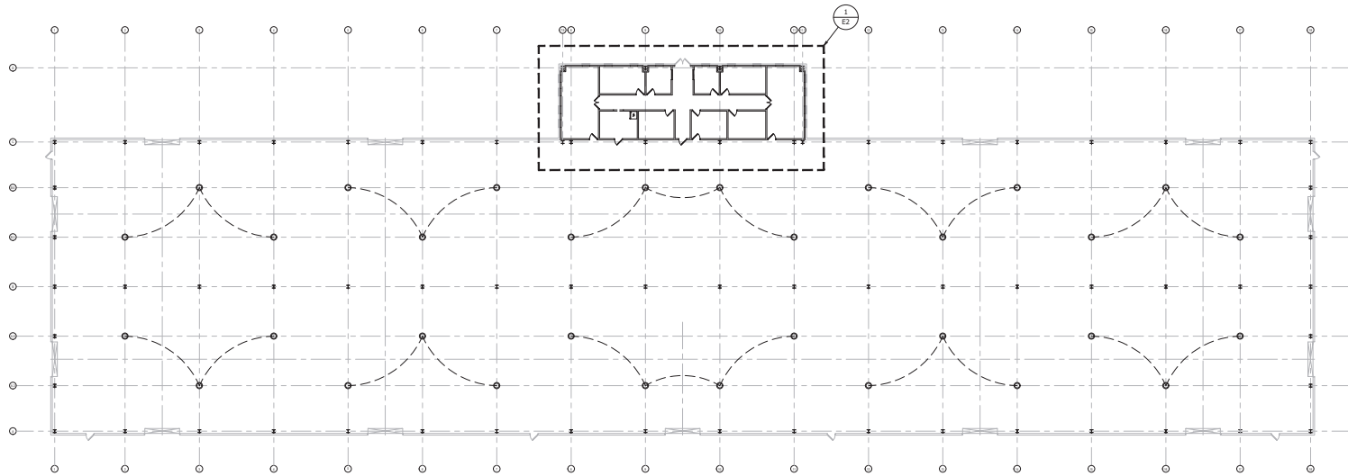
E1 LIGHTING PLAN (WAREHOUSE) SCALE: 1/16"=1'-0"
