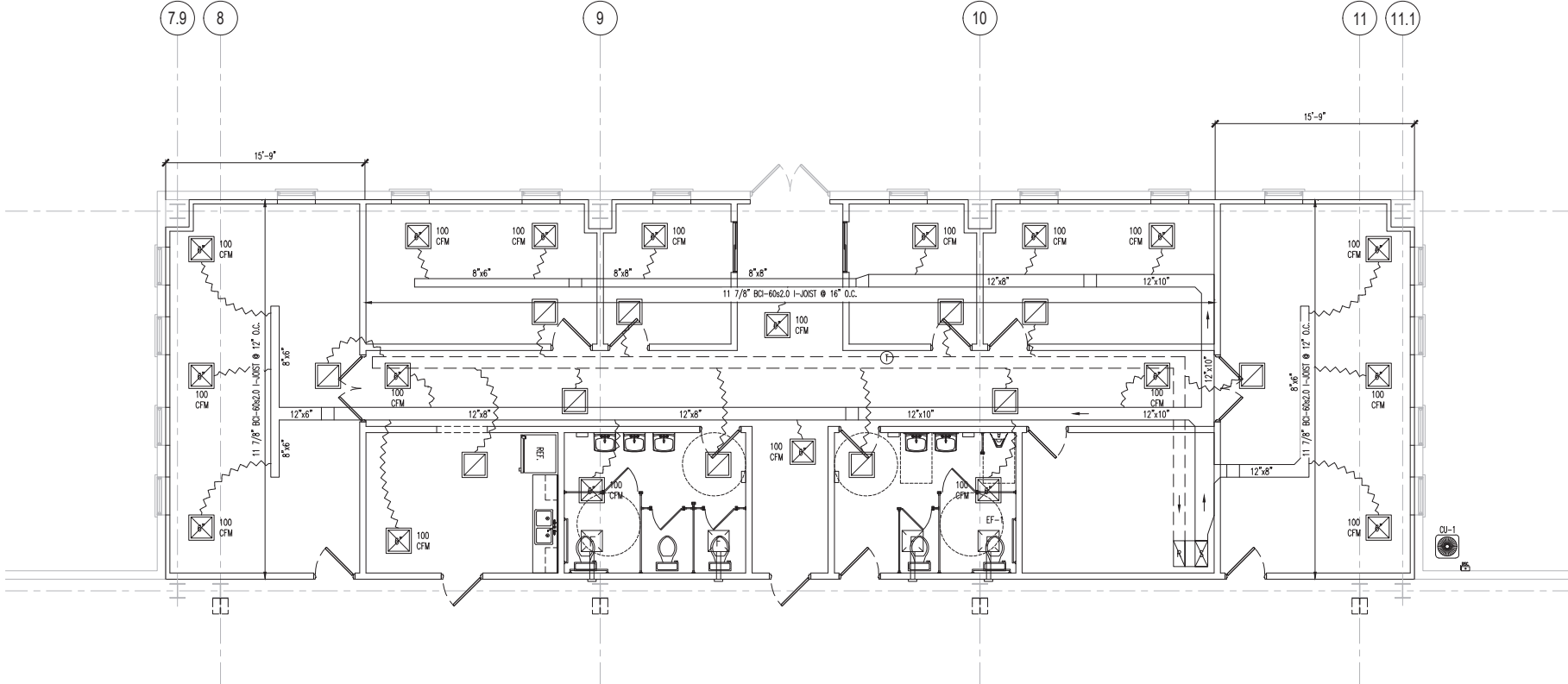
1 MECHANICAL PLAN (OFFICE) M1 SCALE: 1/4"=1'-0"
