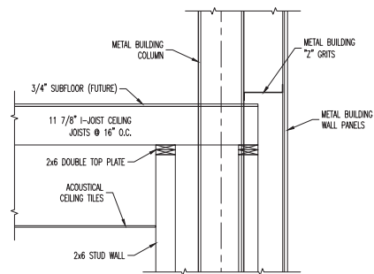
3 CEILING FRAMING DETAIL S3 SCALE: 3/4"=1'-0"
