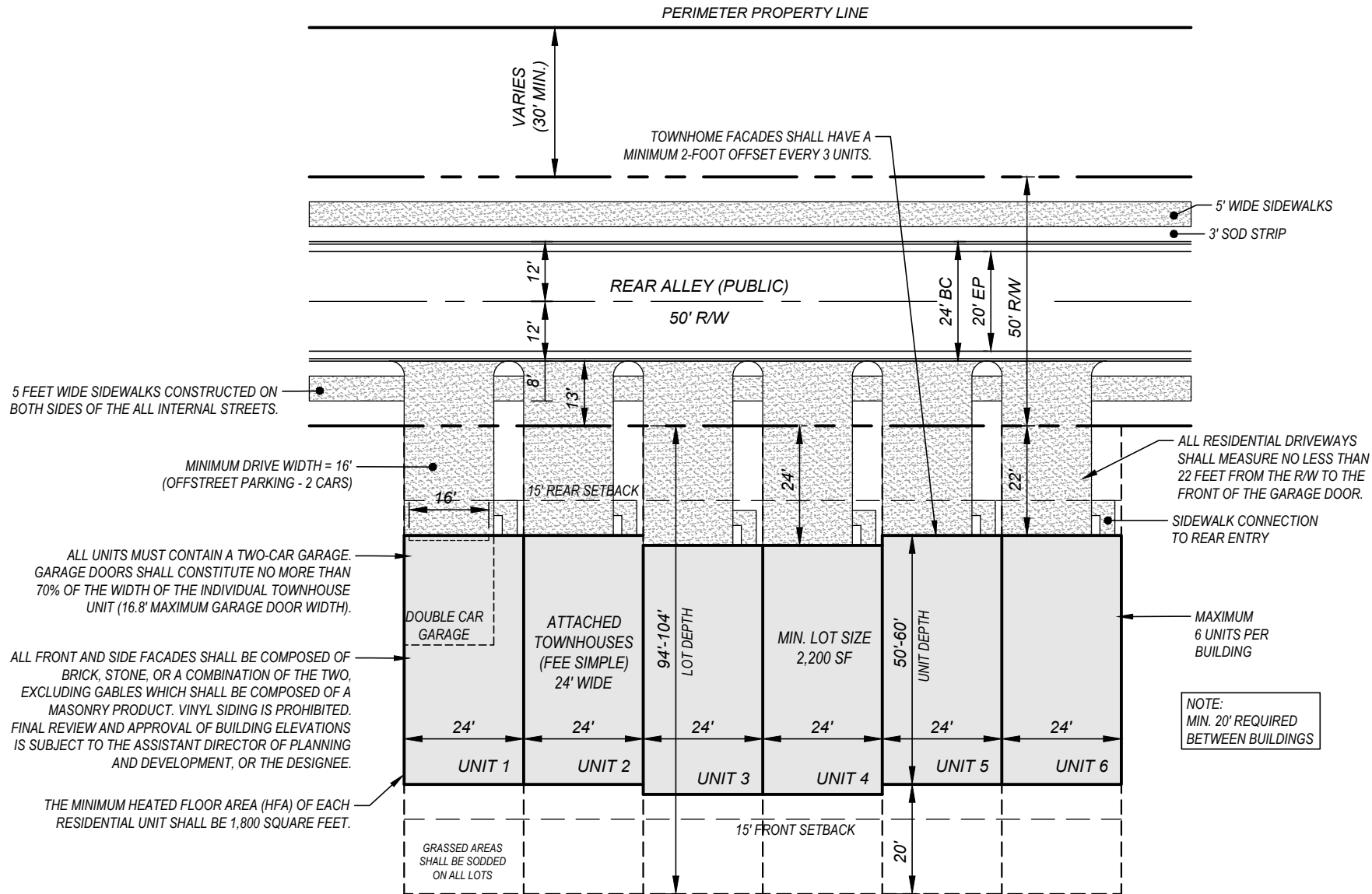
TYPICAL LOT LAYOUT 24' WIDE TOWNHOMES REAR ENTRY
