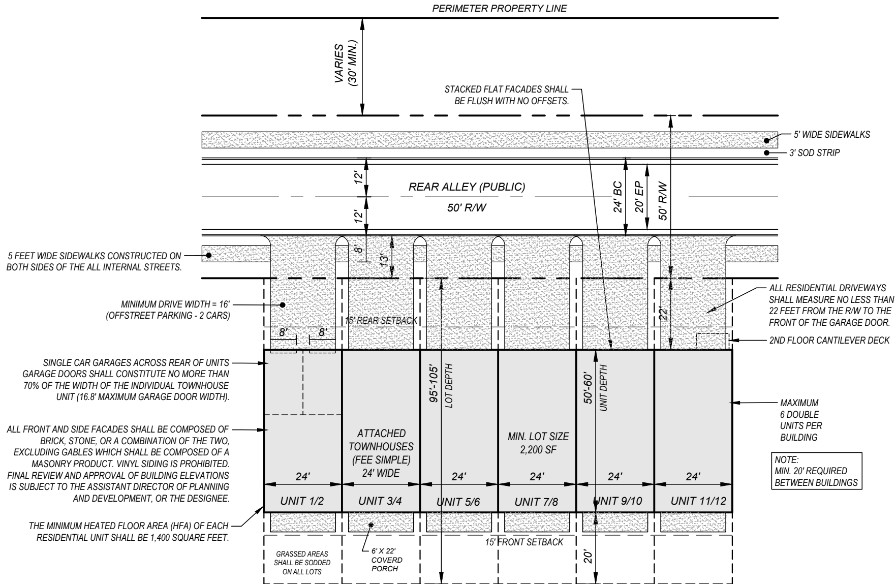
TYPICAL LOT LAYOUT 24' WIDE STACKED FLATS REAR ENTRY
