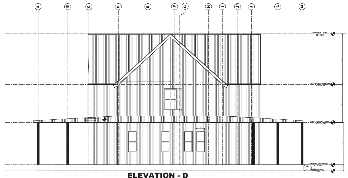
1 A5 ELEVATION-D SCALE 1/4" = 1'-0"
