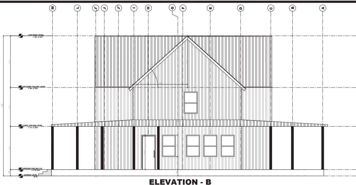
1 A5 ELEVATION-B SCALE 1/4" = 1'-0"
